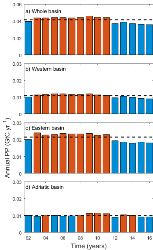
990 Supp Figure 1. Annual coastal variations in \Sigma PP (GtC yr -1 ) for a) the whole Mediterranean Sea, b) the western basin, c) the eastern basin and d) the Adriatic basin. Dash black lines indicate the mean \Sigma PP_{Coastal} for the period 2002-2016 at each study region. Red and blue bars indicate years above and below average values.
