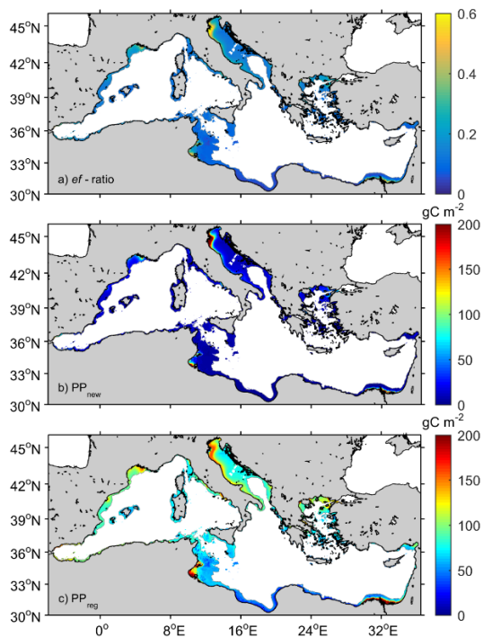
Figure 8. a) ef -ratio in coastal waters (<200 m) of the Mediterranean Sea and estimated values of b) new ( PP_{new} ) and c) regenerated production ( PP_{reg} ). Mean values for the period 2002-2016.
