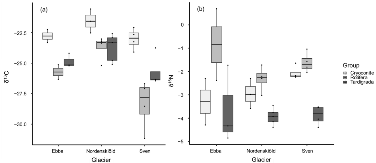
Figure 3. Distribution of \delta^{13}\text{C} (a) and \delta^{15}\text{N} (b) isotopic values in tardigrades (n = 12), rotifers (n = 10) and cryoconite (n = 9) among glaciers. The differences in variances among glaciers are the result of the low number of replicates.
