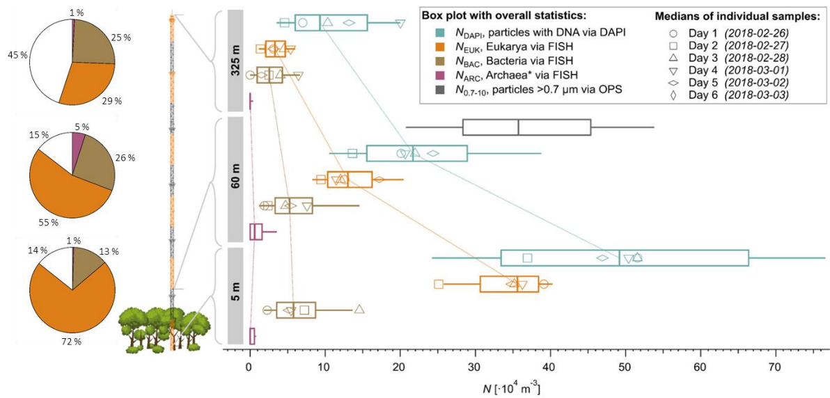
Figure 3: Height profiles of aerosol number concentrations observed at 5 m, 60 m, and 325 m above ground at the ATTO-tower. The median concentrations of all daily samples are displayed as vertical box-whisker plots with 25 and 75 quartiles as box, and 10 and 90 percentiles as whiskers. Daily median values are shown as markers according to the legend. Bioaerosols were quantified with FISH as well as DAPI staining. The total aerosol number concentration at 60 m was determined by an optical particle sizer (OPS) in the corresponding size range.
