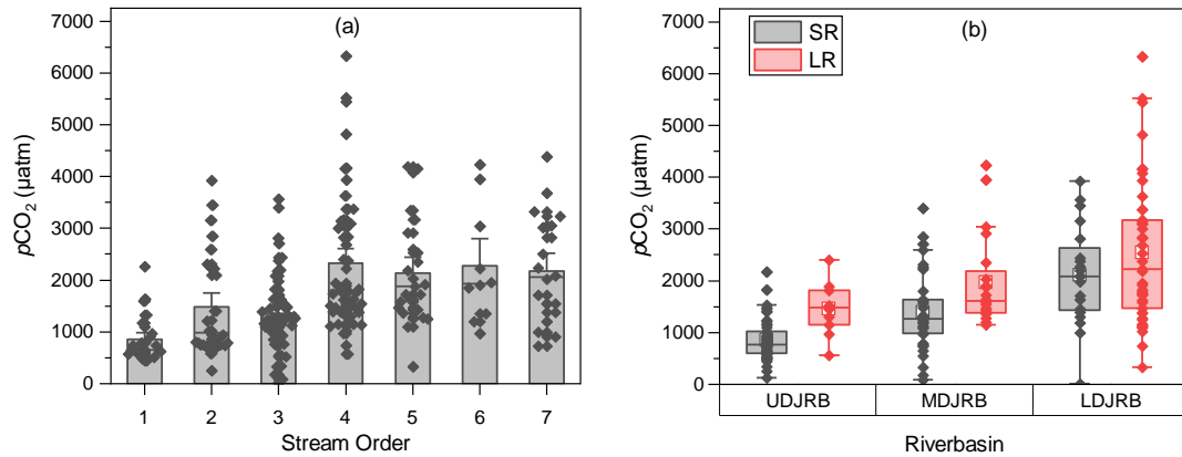
Figure 3 Spatial variations in p\text{CO}_2 . (a) Yearly average p\text{CO}_2 in the seven stream orders, standard errors (SE) are displayed by error bars. (b) Measured p\text{CO}_2 in small and large rivers among three regions in the DJRB. The box mid-lines represent medians; the interquartile range (IQR) is represented by top and bottom of the box, respectively; whiskers indicate the range of 1.5 IQR; the white square symbols represent means, and the other symbols represent p\text{CO}_2 values for each sampled site.
