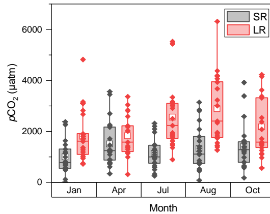
260 Figure 4 Seasonal p\text{CO}_2 changes in small and large rivers. The box mid-lines represent medians; the interquartile range (IQR) is represented by top and bottom of the box, respectively; whiskers indicate the range of 1.5 IQR; the white square symbols represent means, and the other symbols represent p\text{CO}_2 values for each sampled site.
