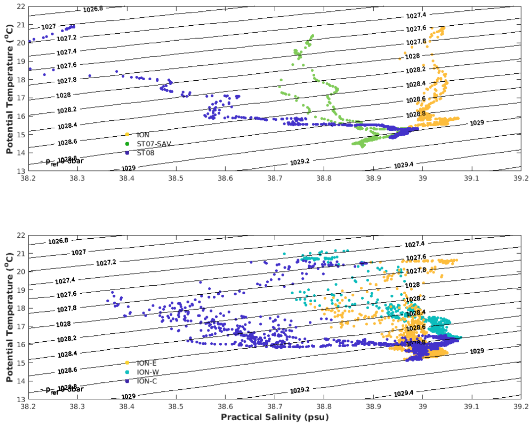
Figure 6. TS-diagram for stations ION, SAV, ST7, ST8 restricted to 0-300m (top) and for ION-Tr parts (bottom), ION-W, ION-C, ION-E.
