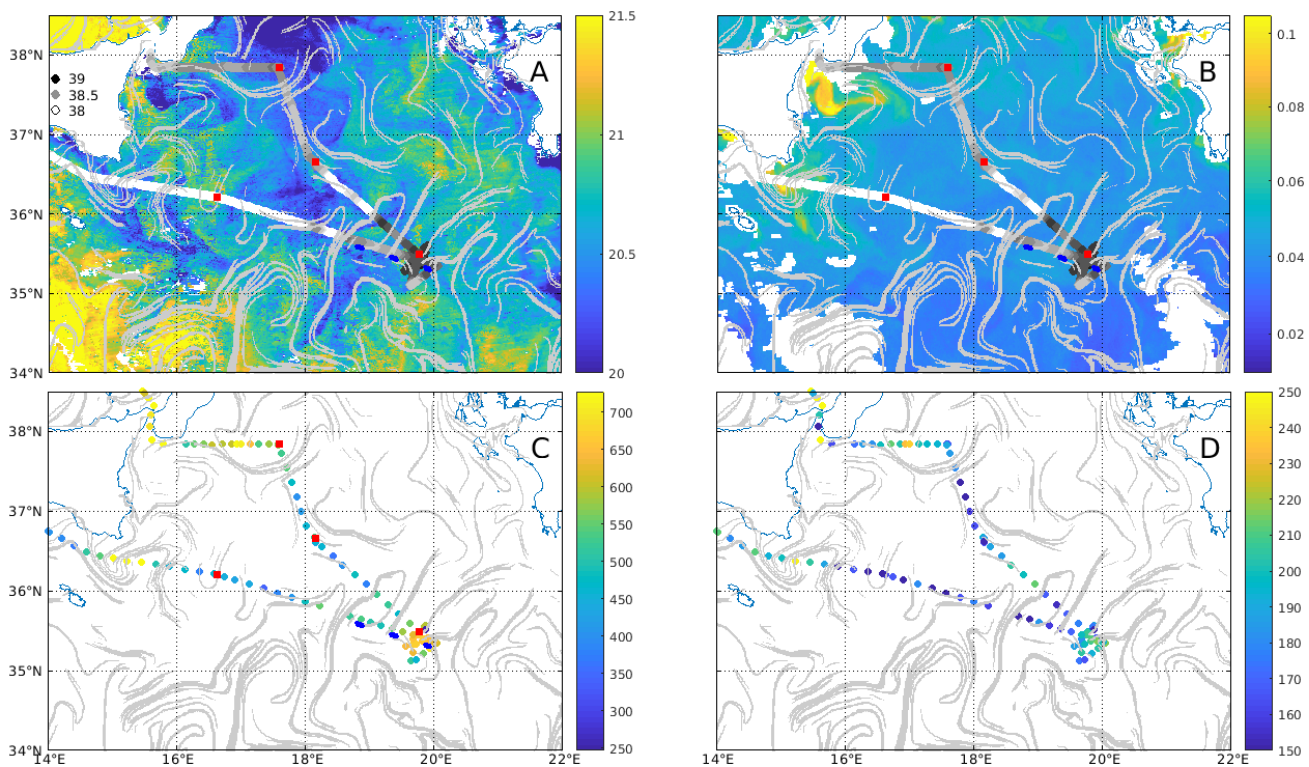
635 Figure 3. A) Satellite SST (May 29-30 th , night, °C). B) Chl-a (May 30 th , mg/m 3 ). On panels A and B, underway surface salinity from TSG is overlaid as dots, darker for saltier water. C) Underway surface abundance (cells.cm -3 ) of nanoeukaryotes1 group from cytometry. D) Underway surface abundance (cells.cm -3 ) of coccolithophore like group from cytometry. On all panels, FSLE ridges are overlaid in light grey (>0,15 day -1 ). Stations positions are marked as red squares and ION-Tr parts as blue dots as figure 1.
