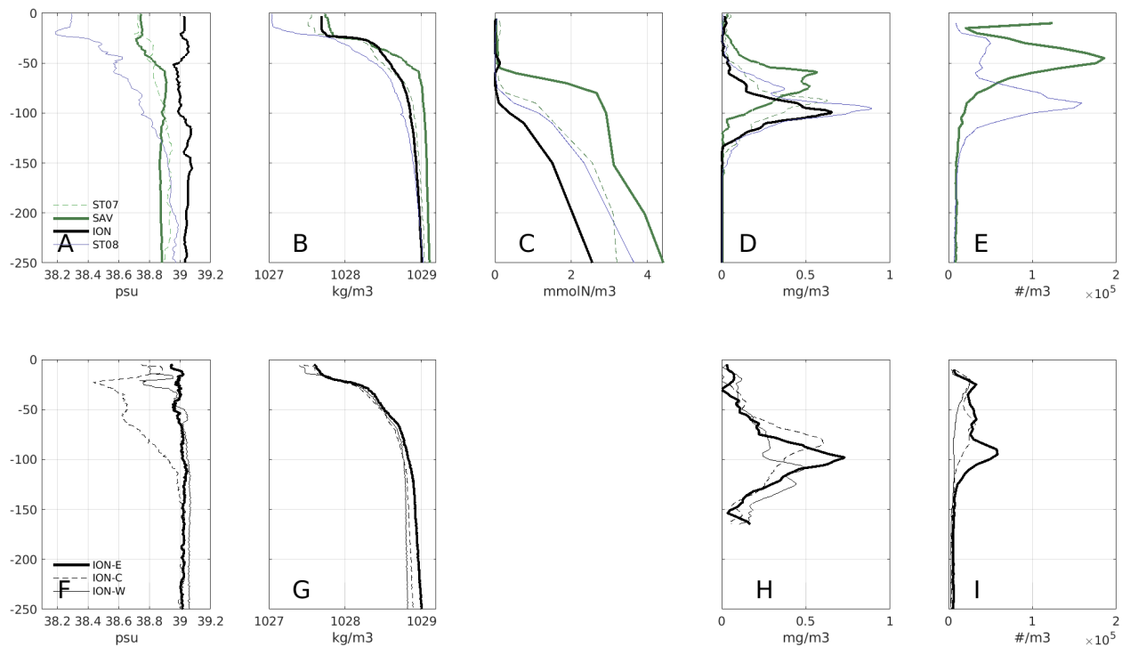
Figure 7. Vertical profiles of variables at ION, SAV, ST7, ST8 (top) and for ION Tr parts (bottom), ION-W, ION-C, ION-E. Panels A and F Salinity, B and G density, C Nitrate, D and H Chl-a, E and I total particle abundance. Note that particles were not quantified at ST7.
