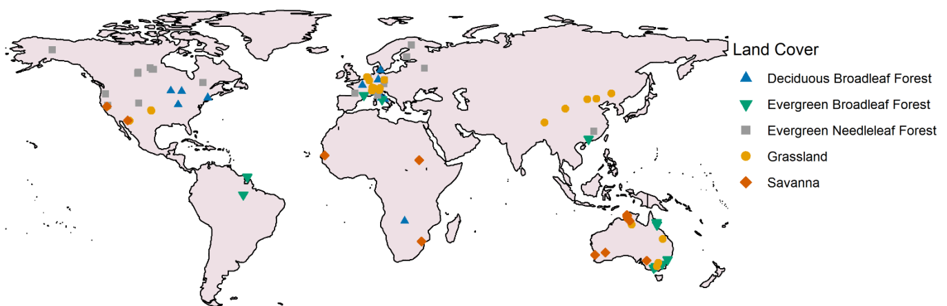
Figure 2 Location and vegetation type of the 93 included flux tower sites.
