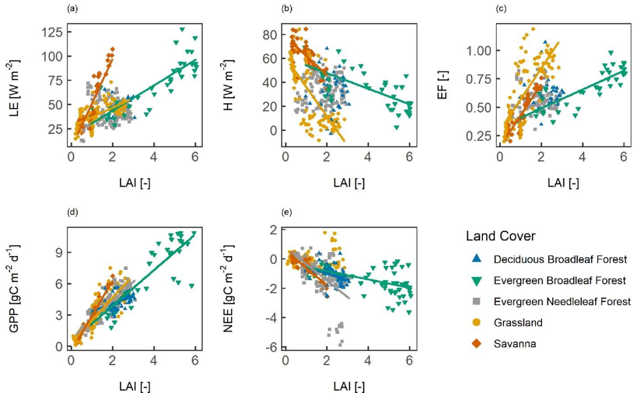
Figure 4 The spatio-temporal correlation between surface fluxes and leaf area index (LAI). Panels show (a) the latent heat flux (LE), (b) the sensible heat flux (H), (c) the evaporative fraction (EF), (d) gross primary productivity (GPP), and (e) net ecosystem exchange (NEE). A line indicates a significant correlation at p < 0.05 .
