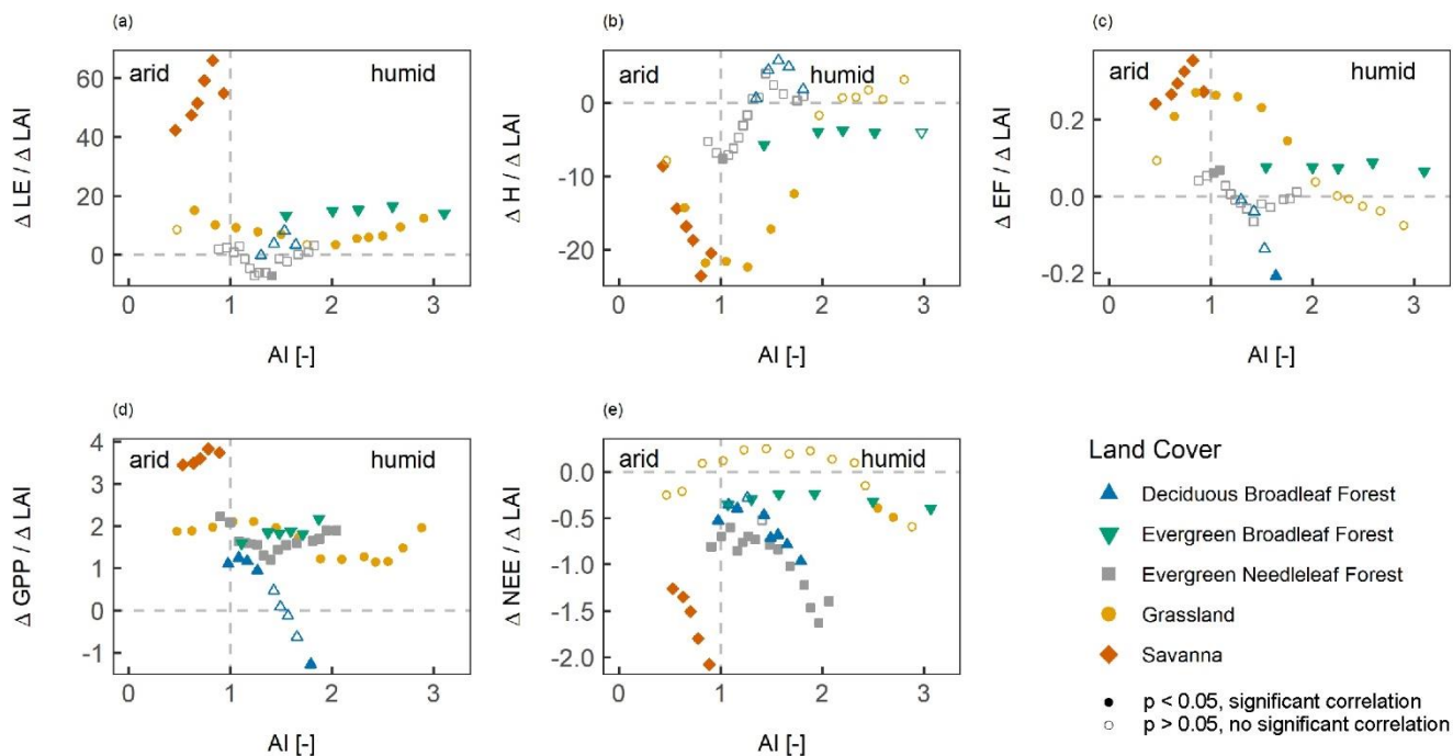
Figure 7 The effect of aridity on the relation between surface fluxes and leaf area index (LAI). The slope of the correlation between LAI and surface fluxes is shown for different aridity values for (a) the latent heat flux (LE), (b) the sensible heat flux (H), (c) the evaporative fraction (EF), (d) gross primary productivity (GPP), and (e) net ecosystem exchange (NEE). Each dot indicates the slope value for the 30 closest aridity values. The filled symbols indicate that the correlation was significant at p < 0.05 , while the empty symbols indicate a non-significant correlation.
