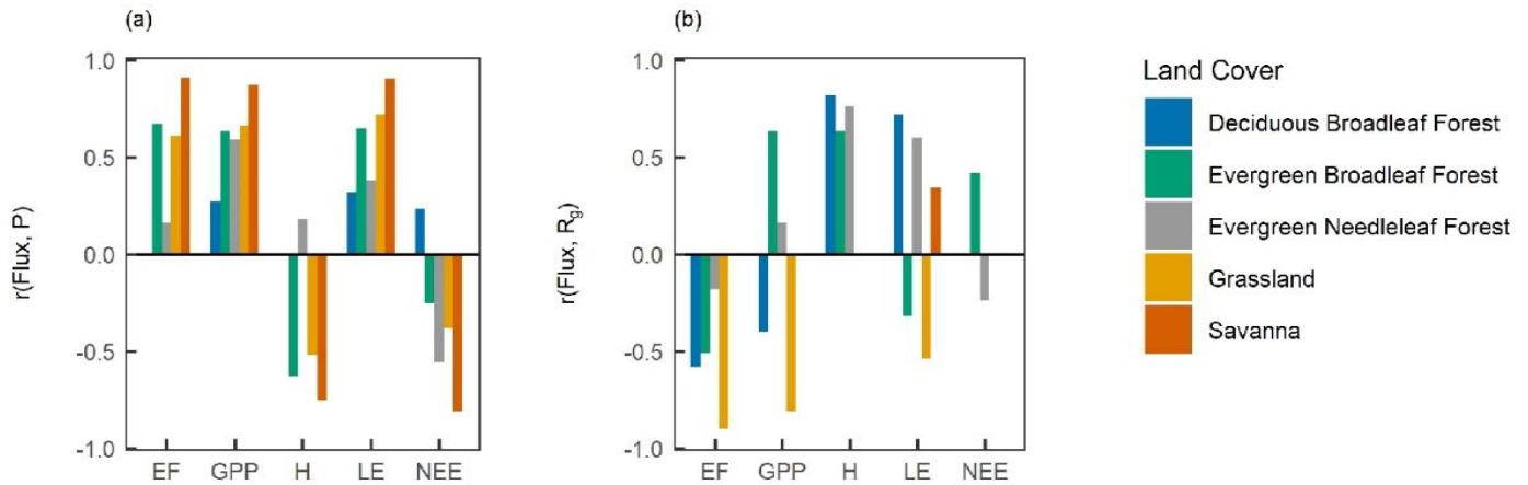
Figure 8 Water and energy control on surface fluxes. The correlation coefficient ( r ) between site-year surface fluxes versus (a) mean yearly precipitation ( P ) and (b) incoming shortwave radiation ( R_g ). Each bar indicates a significant correlation at p < 0.05 .
