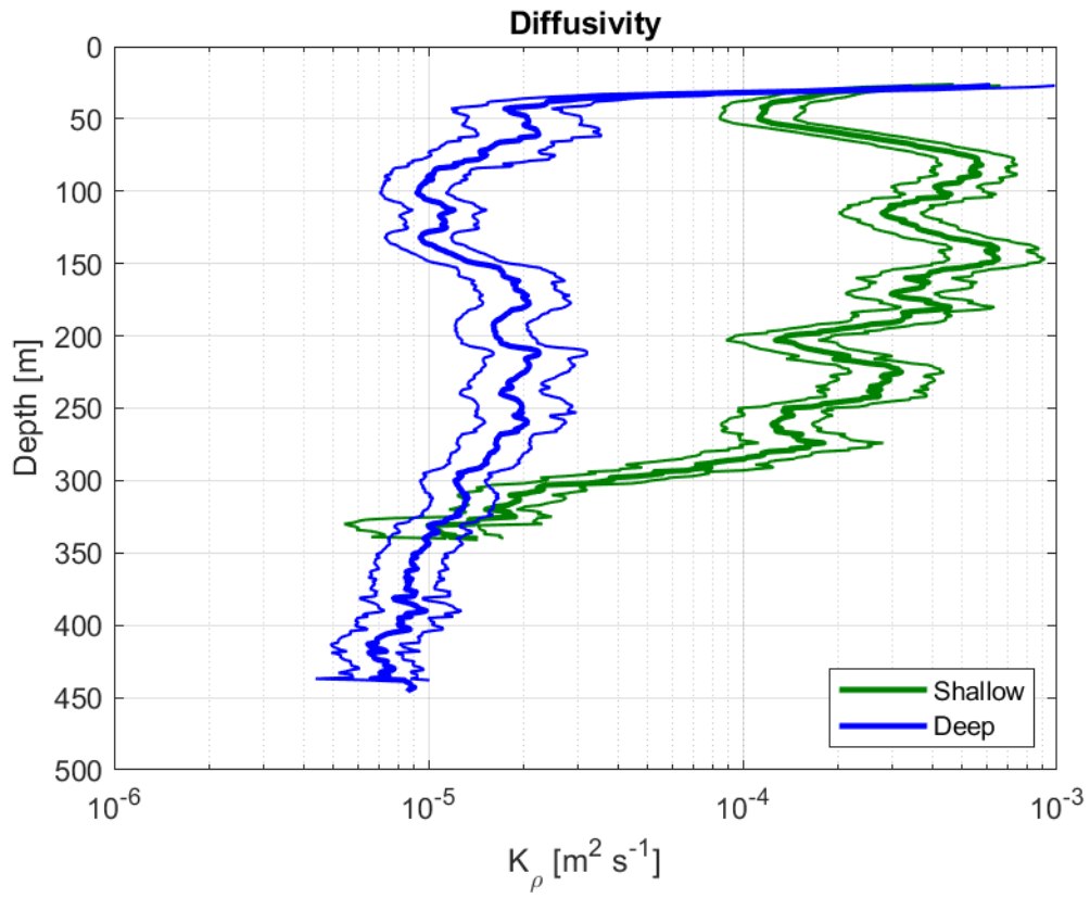
Figure S1. Diffusivities averaged over cruises M136 and M137 for both the shallow (bottom depth < 500 m; green) and deep (bottom depth > 500 m; blue) stations.
