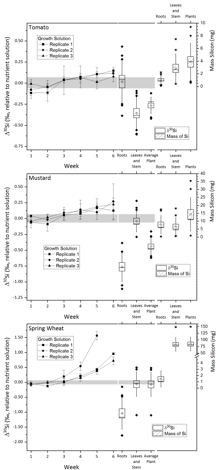
Figure 2: Silicon isotope composition (left) and mass of silicon taken up (right) during the growth of tomato (top panel), mustard (mid-panel) and wheat (bottom panel). On the left y-axis shows the \delta^{30}\text{Si} composition in ‰ relative to the nutrient solution, is reported, on the right y-axis the mass of silicon incorporated by the plants in mg incorporated by the plants. The line connects \delta^{30}\text{Si} from the weekly sampled nutrient solution (week 1 to 6). The box plots denote \delta^{30}\text{Si} (left) and plant organ Mg mass (right), per species 12 roots and 12 leaves and stem samples were analysed, plant averages were weighted by organ mass (calculated using Eq. (2)). Uncertainty bars are based on 2 standard uncertainties, grey bar area is denotes the silicon isotopic composition of the starting solution \pm two standard deviations. The All box sizes is denote one standard uncertainty, vertical-horizontal line in the box is shows the median, empty diamond/stars in the box indicate the mean and filed diamonds/stars are show outliers, outside of one standard deviation. Line plot is the weekly sampled nutrient solution (from week 1 to 6), the box plots are the plant samples, per species 12 roots and 12 leaves and stem samples were analysed, average were weighted by organ mass (calculated using Eq. (2)).
