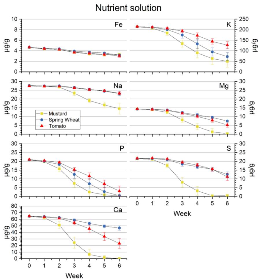
15 Figure S 1: Temporal evolution of nutrient concentrations during the hydroponic growth of the different plant species. Concentration (Fe, K, Mg, Ca, P, S, Na in \mu\text{g}\cdot\text{g}^{-1} ) are based on the mean of the three replicated containers, uncertainty shown is 1 standard deviation of those replicated containers.
