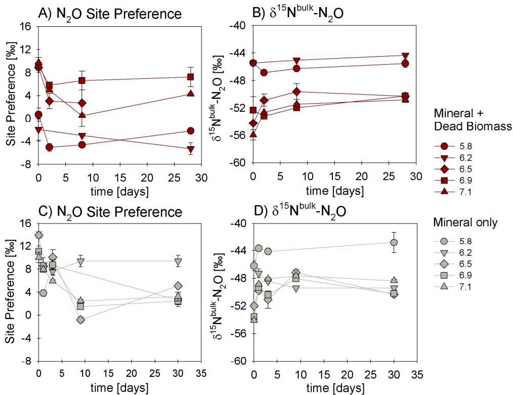
Fig. 2. Site Preference (SP; A, C) and \delta^{15}\text{N}^{\text{bulk}}\text{-N}_2\text{O} (B, D) values of \text{N}_2\text{O} produced in experiments amended with mineral + dead biomass (red) and mineral-only (grey)
