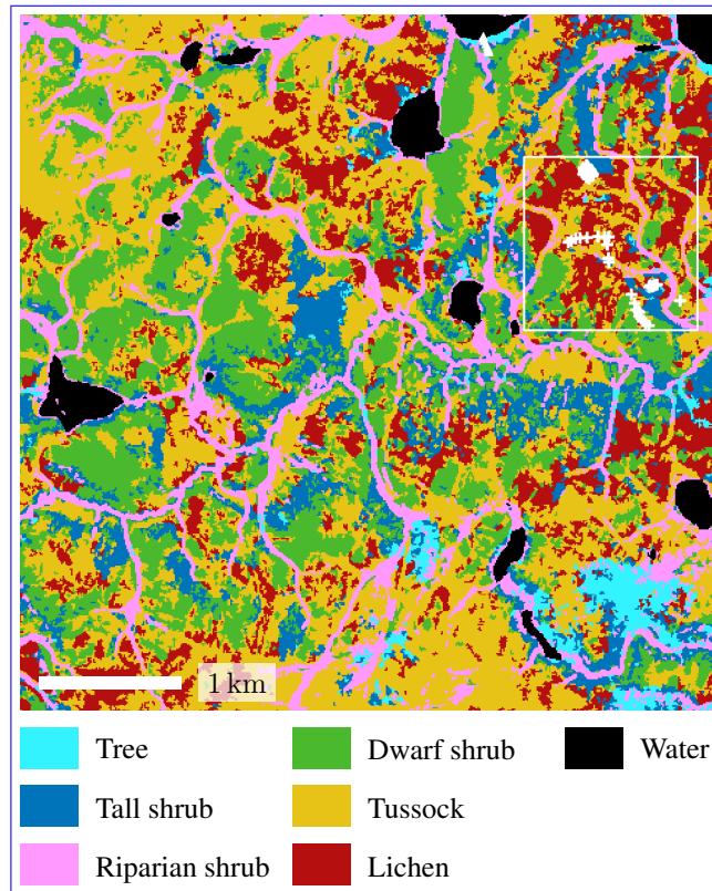
Figure 2. Vegetation map of the study region using the vegetation types as described above (Grünberg and Boike, 2019); the map is based on airborne orthophotos and vegetation height derived from airborne laser scanning (Anders et al., 2018); the white square indicates the study site extent including all sensor locations (white plus signs) as shown in Figure 1b.
