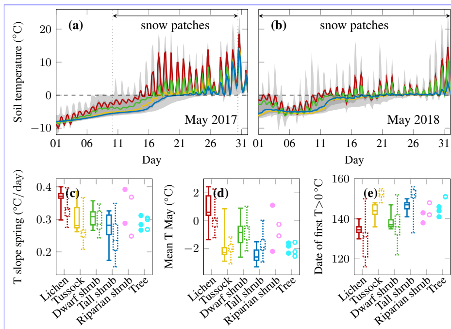
Figure 8. Topsoil temperature series of (a) May 2017 and (b) May 2018 representing spring of the two different measurement periods; mean of all measurements below four different vegetation types is shown in colour, the range of all single sensors is shown in light grey, and the range of all sensors between the 10th and 90th percentile is shown in darker grey; boxplots of all measurements per vegetation type are represented by boxes of the first period on the left and the second period on the right and dotted; for riparian shrubs and trees all single observations are shown with filled symbols for the first period and open symbols for the second; (c) rate of warming in spring; (d) mean May temperature; (e) date when thawing is complete.
