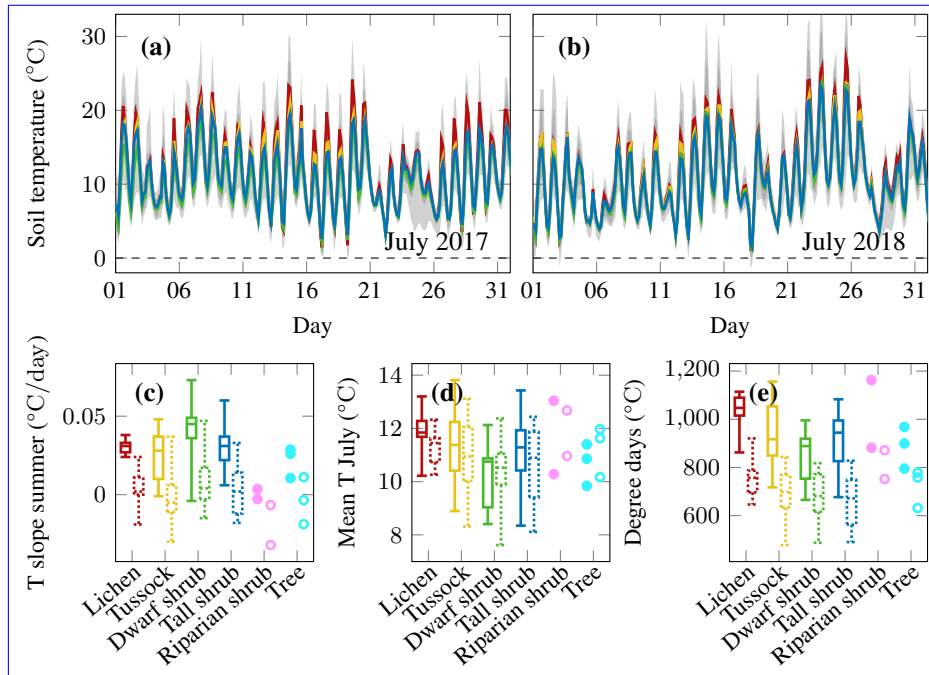
Figure 9. Topsoil temperature series of (a) July 2017 and (b) July 2018 representing summer of the two different measurement periods; mean of all measurements below the four different vegetation types is shown in colour, the range of all single sensors is shown in light grey, and the range of all sensors between the 10th and 90th percentile is shown in darker grey; boxplots show all measurements per vegetation type with boxes of the first period on the left and the second period on the right and dotted; for riparian shrubs and trees all single observations are shown with filled symbols for the first period and open symbols for the second; (c) rate of warming in summer; (d) mean July temperature; (e) cumulative sum of positive degree days until the end of August.
