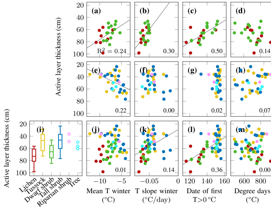
Figure 10. The relationship between active layer thickness at the end of August 2018 and (i) vegetation type; (a, e, j) mean topsoil winter temperature; (b, f, k) rate of topsoil cooling in winter; (c, g, l) day of the year when the topsoil warms above 0 °C; (d, h, m) cumulative sum of positive degree days until the end of August of the same year; top row: lichen and dwarf shrub tundra; middle row: tussock, tall shrub, riparian shrub, and tree; bottom row: all vegetation types; the numbers indicate the Pearson's correlation coefficient R^2 ; the thin grey lines are regression lines of significant ( p < 0.05 ) relationships.
