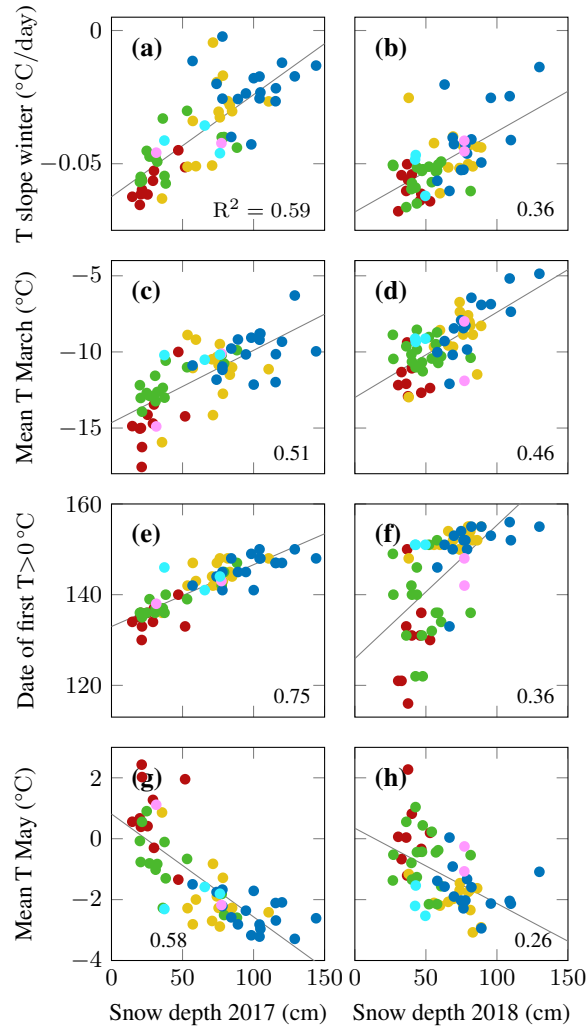
Figure 7. The relationship between snow depth end of April 2017 (left column) and 2018 (right column) and (a, b) rate of cooling in winter; (c, d) mean temperature in March; (e, f) day of year when the topsoil warms above 0 °C; (g, h) mean temperature in May; the symbol colours refer to different vegetation types (see e.g. Figure 6); the numbers indicate the Pearson's correlation coefficient R^2 ; the thin lines are regression lines of significant ( p < 0.05 ) relationships.
