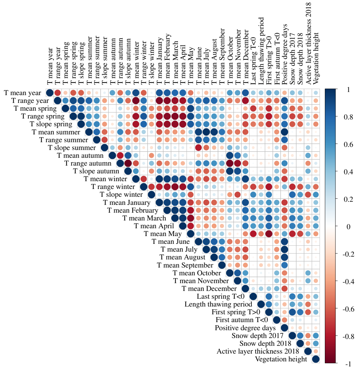
Figure 3. Pearson's correlation coefficients (R) of all topsoil temperature characteristics ( ^{\circ}\text{C} ), active layer thickness (cm), and snow depth (cm) in the first period (September 2016 to August 2017).
