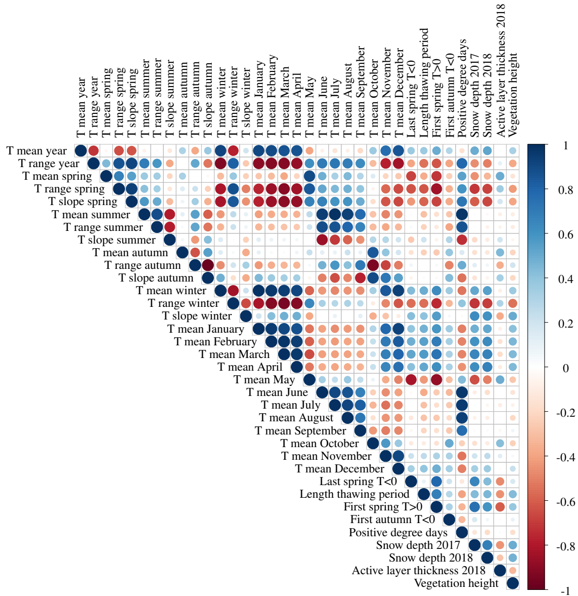
Figure 4. Pearson's correlation coefficients (R) of all topsoil temperature characteristics ( ^{\circ}\text{C} ), active layer thickness (cm), and snow depth (cm) in the second period (September 2017 to August 2018).
