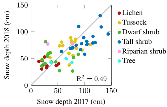
Figure B2. Snow depth measured at the end of April in 2017 and 2018 at approximately the same locations; the number indicates the Pearson's correlation coefficient R^2 ; the grey line is the 1:1 line.
