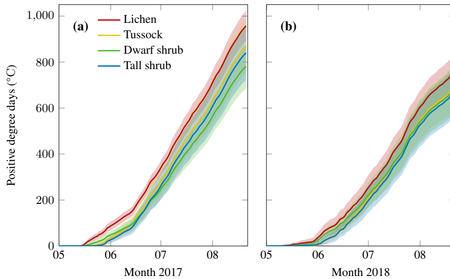
Figure B3. Cumulative positive degree days of topsoil temperature below different vegetation types; the lines indicate the mean of all series per type, the shaded areas represent the mean plus/minus the standard deviation; (a) 2017, (b) 2018.
