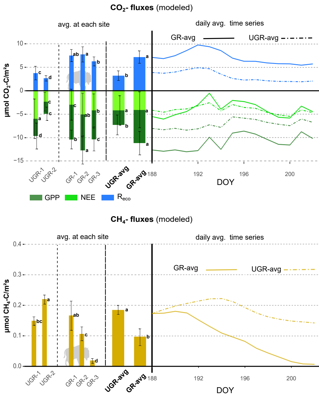
Figure 2. Overview on C-fluxes at all chamber plots from July 7th to July 21st. Differing letters indicate significant differences between plots ( p < 0.01 , please see also Table B3 for details). Overall (site average), NEE did not differ significantly between GR and UGR, while GPP and R_{eco} were significantly larger at GR. Daily average CH_4 emissions at grazed plots strongly decrease over time, leading to a substantial net reduction in methane emissions at the GR plots, compared to the UGR reference.
