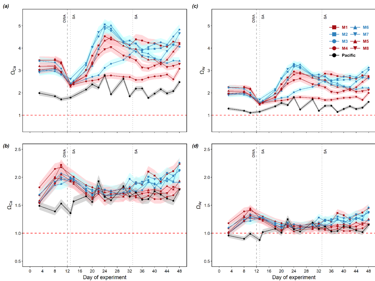
306 Figure 4 Temporal dynamics of depth-integrated surface calcite saturation state (a), bottom calcite saturation state (b), surface 307 aragonite saturation state (c), and bottom aragonite saturation state (d) in the mesocosms and the surrounding Pacific. The error 308 ribbons present the propagated standard uncertainties of the calculations. When \Omega > 1 (above red dashed line), seawater is 309 supersaturated for calcium carbonate. When \Omega < 1 (below red dashed line), seawater is under-saturated for calcium carbonate. 310 Color codes and symbols denote the respective mesocosm. Abbreviation: OWA, OMZ water addition. SA, salt addition.
