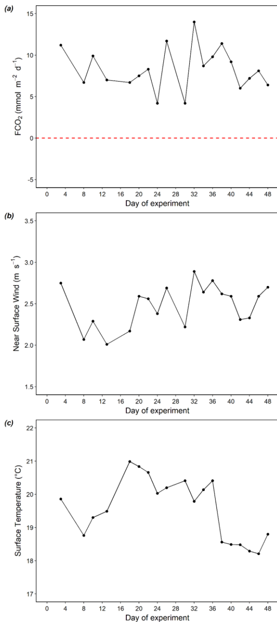
320 Figure 5 Temporal dynamics of surface air-sea CO_2 flux (a), near surface wind speed (b) and surface temperature (c) in the Pacific. 321 FCO_2 > 0 (above red dashed line) indicates CO_2 outgassing from the sea surface to the atmosphere. FCO_2 < 0 (below red dashed 322 line) indicates a CO_2 flux from the atmosphere to the sea.
