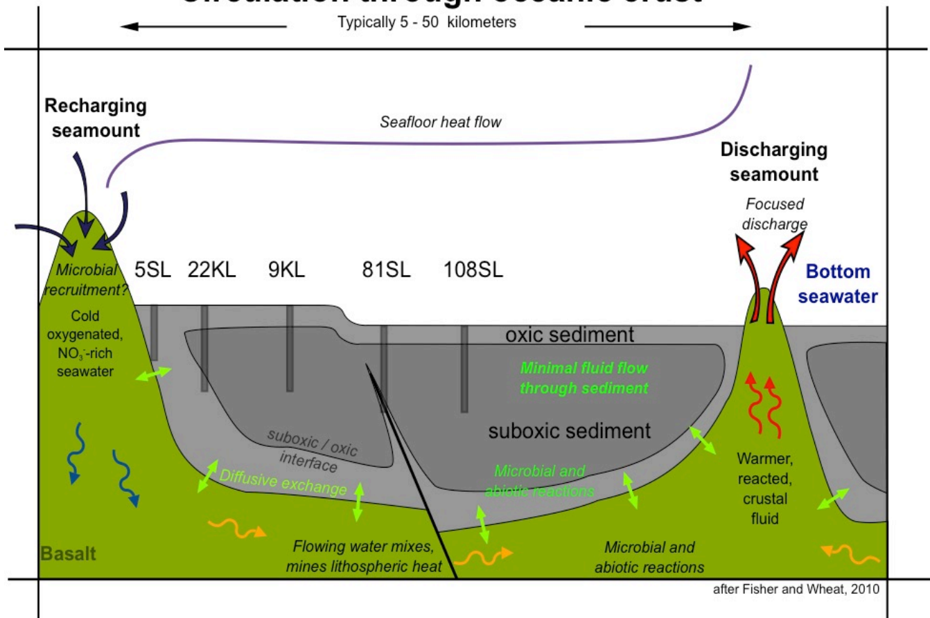
835 Figure 7: Model of fluid circulation in the basaltic basement, diffusive exchange with the sediment and the sediment oxidation state. Note the influence of faults. Representative cores taken during SO240 are placed such that their geochemical profiles match with the model (modified from Fisher and Wheat, 2010).
