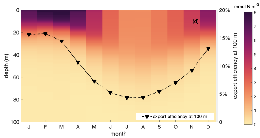
Figure 1: Organic matter ( \text{mmol N m}^{-3} ) depth-month distribution with the seasonal cycle of export efficiency at 100 m (black triangle) within the focus region.
