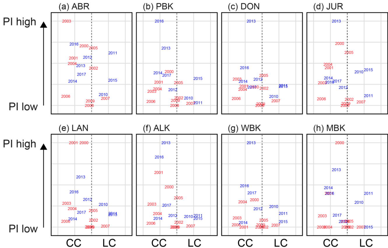
515 Figure 14 Relationship of the more dominant current during the late summer/early autumn (December - March) to late PI at monitoring sites (a) Abrolhos (b) Port Gregory (c) Dongara (d) Jurien Bay (e) Lancelin (f) Alkimos (g) Warnbro and (h) Cape Mentelle. The x-axis is the difference between the LC and CC standardised, indicating which is more prominent at the time. Red indicates the seasons before the recruitment failure; blue indicates seasons after.
