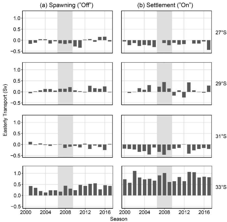
335 Figure 7 Cross-shelf transport (easterly) between 200 - 50 meters over 2-degree latitudinal bins (26-28° S, 28-30° S, 30-32° S and 32- 34° S). Averaged for the (a) spawning “off” transport season (September-February, season -1) and (b) settlement “on” transport season when variation in cross-shelf transport is the highest (April-September). Grey shaded seasons (2008 and 2009) indicate the less than expected PI based on a priori relationships (Caputi et al. 2001).
