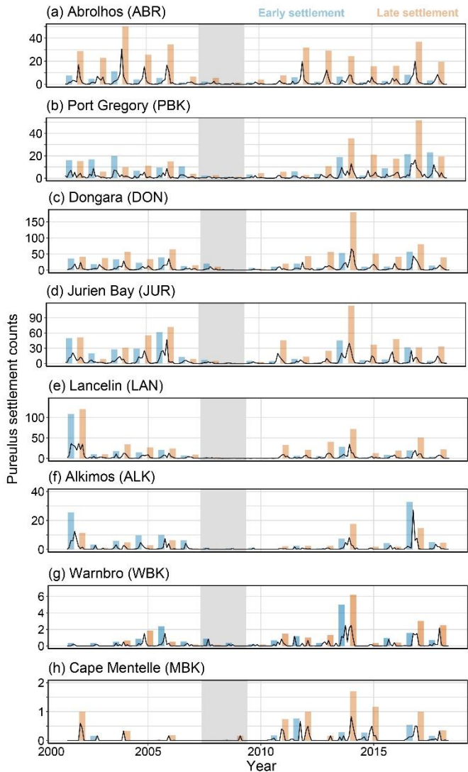
285 Figure 4 Monthly average puerulus counts for each monitoring site (black line) with the early (May - October, blue) and late (November - April, red) puerulus settlement for the season. The index is a sum of the included monthly average puerulus counts. Grey shaded seasons (2008 and 2009) indicate the less than expected PI based on a priori relationships (Caputi et al. 2001).
