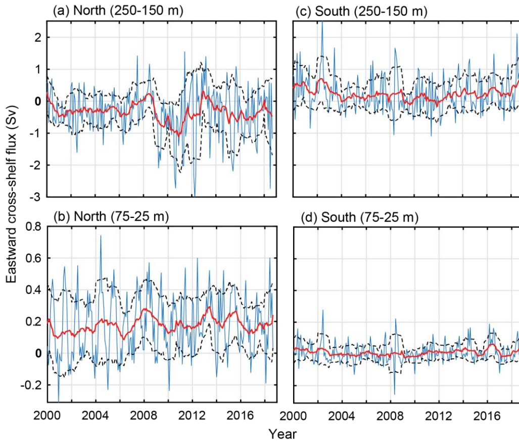
Figure 12 Cross-shelf transport (easterly) between 2000 and 2018 off the shelf. North and south divide are shown in Figure 1a. (a) North cross-shelf flux between 250-150 m and (b) 75-25 m. (c) South cross-shelf flux between 250-150 m and (d) 75-25 m. The yearly moving mean (red) and the positive and negative moving standard deviation (dashed black) are included.
