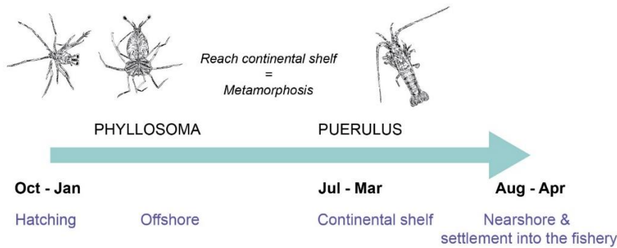
Figure 1 Early life-cycle schematic of P. cygnus . Below the arrow indicates each stage's approximate timing (black) and location (blue). Above the arrow displays their growth, image credit Alice Ford.
