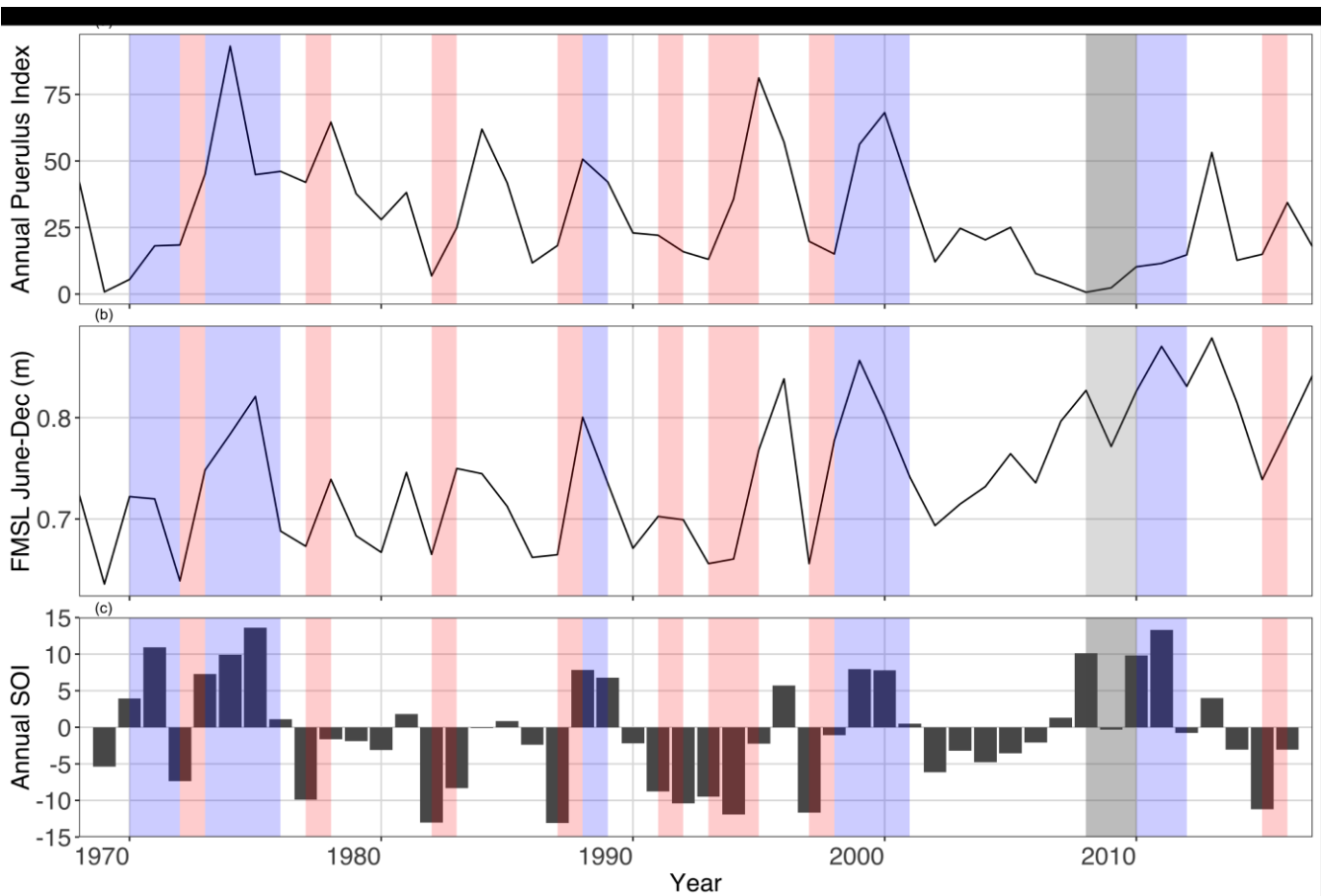
85 Figure 3 Time series of annual (a) fishery-wide PI (May – April); (b) Fremantle Mean Sea Level (FMSL) over June to December (m); and, (c) Southern Oscillation Index (SOI) (May –April). Grey shaded seasons indicate the less than expected PI based on a priori relationships (Caputi et al. 2001). Blue and red shading indicate a La Niña and El Niño periods, respectively. Updated to 2018 and modified from Figure 5 in Caputi et al. 2001.
