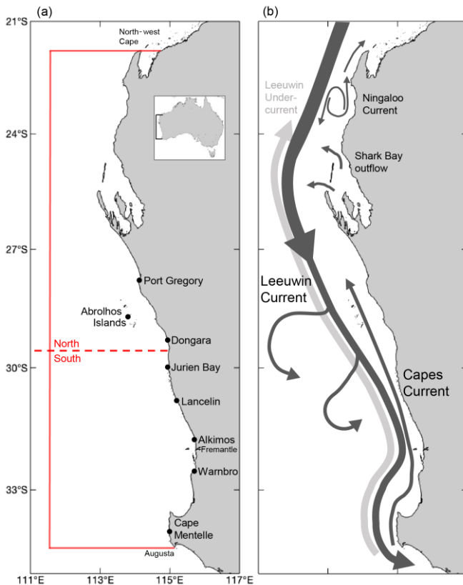
Figure 2 (a) Locations of puerulus survey sites included within this study and other locations of note. The north and south refer to the midpoint used in this analysis. Red boundary is the extent of environmental variables. Inset shows location of the coastline in
