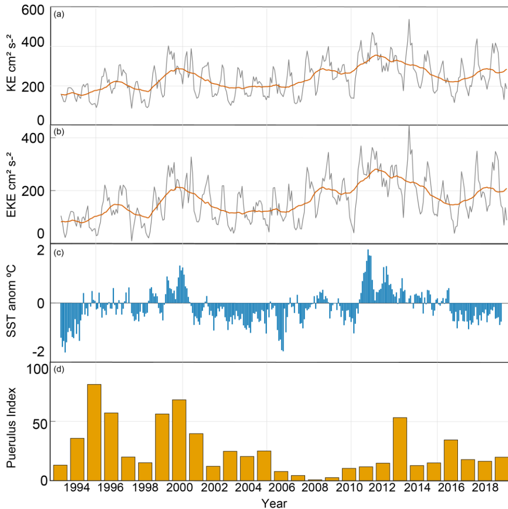
Figure 11 (a) Kinetic energy and (b) eddy kinetic energy ( \text{cm}^2 \text{s}^{-2} ) from altimeter data, the (c) SST ( ^{\circ}\text{C} ) anomaly from SSTAARS and (d) PI for the whole Western rock lobster fishery.
