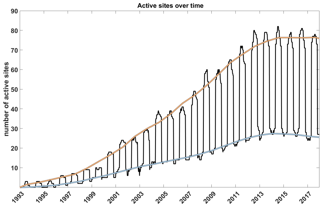
335 Figure 2: Development of eddy-covariance network data coverage at monthly time steps. The fluctuating black line gives the total number of active sites per month, orange and light blue lines indicating the long-term development of data coverage during summer and winter, respectively. For sites from our dataset where activity was only specified per year, summertime-only data coverage was assumed.
