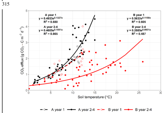
315 Figure 4 Figure 5. Exponential relationship between soil CO 2 effluxes and soil temperature at 2 cm depth measured from area A (mature spruce stand, black) and area B (clearfell site, red), before (dashed lines, 'yr1') and after (solid lines, 'yr2-4') felling. Equations and R 2 for fitted lines shown.
