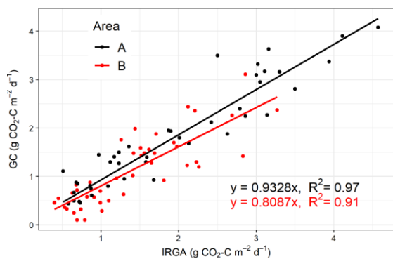
790 Figure S1.2. Comparison between mean CO 2 effluxes measured by gas chromatograph (GC) from the 8 static chambers in each forest area (A = mature stand, B = clearfell) and mean CO 2 effluxes measured by infra-red gas analyser (IRGA), from 25 static chambers in the same areas. The regression intercepts were not significantly different from zero, so the regression was through the origin. The RMSE values were 0.37 and 0.41 g CO 2 -C m -2 d -1 for area A and area B respectively.
