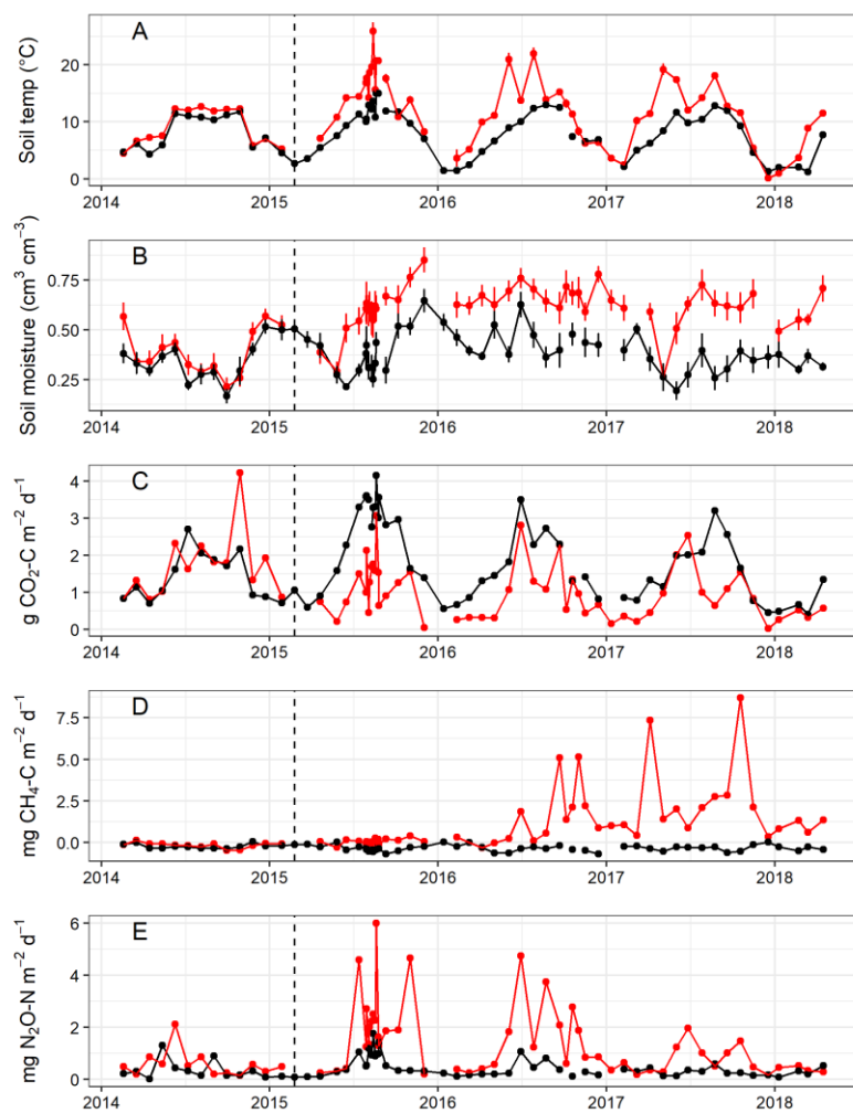
Figure 2. Figure 3. Mean soil temperature (°C) at 2 cm depth (a), volumetric soil moisture content (cm 3 cm -3 ) (b), and median soil CO 2 (c), CH 4 (d), and N 2 O (e) fluxes measured from 8 chambers per area approximately monthly throughout the experiment in Harwood Forest. Black symbols and lines are for area A, (mature spruce stand, remaining) and red are for area B, (mature spruce stand, clearfelled after one year) as indicated by the dotted vertical line. Error bars are standard error of mean of 8 replicate measurements of the soil temperatures and moisture.
