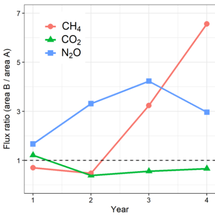
535 Figure 7. Ratios of annual soil GHG fluxes in area B (mature stand, clearfell area, felled after year 1) to that in area A (mature spruce stand, remaining) in Harwood Forest. Note: CH 4 fluxes presented as absolute values. Dashed line is for ratio = 1 (no difference between areas).
