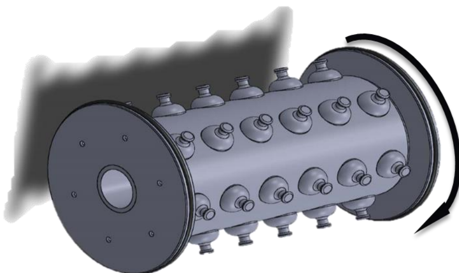
Figure S9. Schematic diagram of rotator used for particle suspension in 2015.
