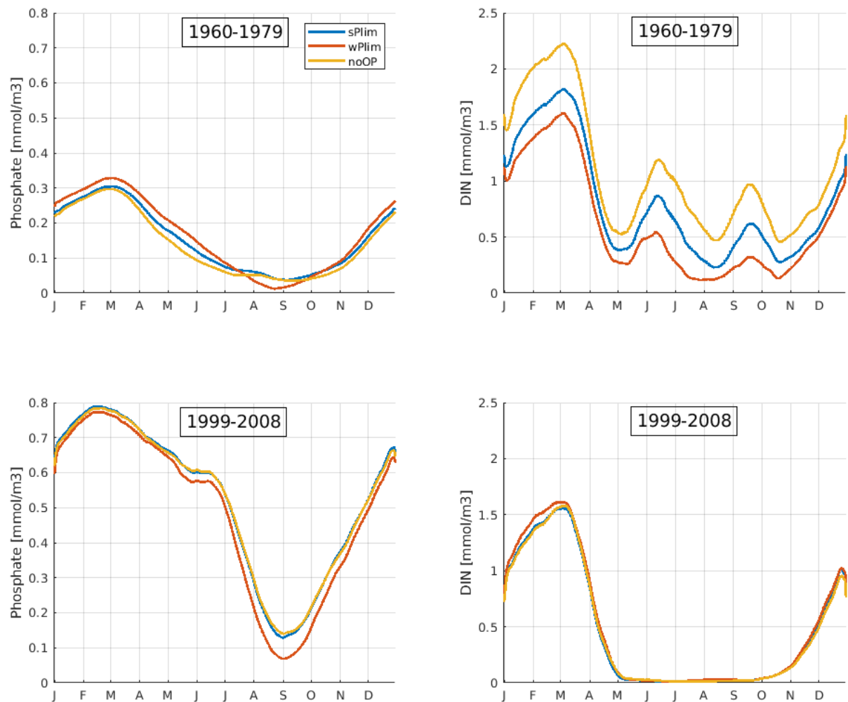
685 Figure 6. SCOBIC-CLC results of the mean seasonal cycles of surface phosphate (left) and dissolved inorganic nitrogen; DIN (right) at station BY15 for the period 1960-1979 (upper) and 1999-2008 (lower). The data-points have been smoothed using a 1 month moving average.
