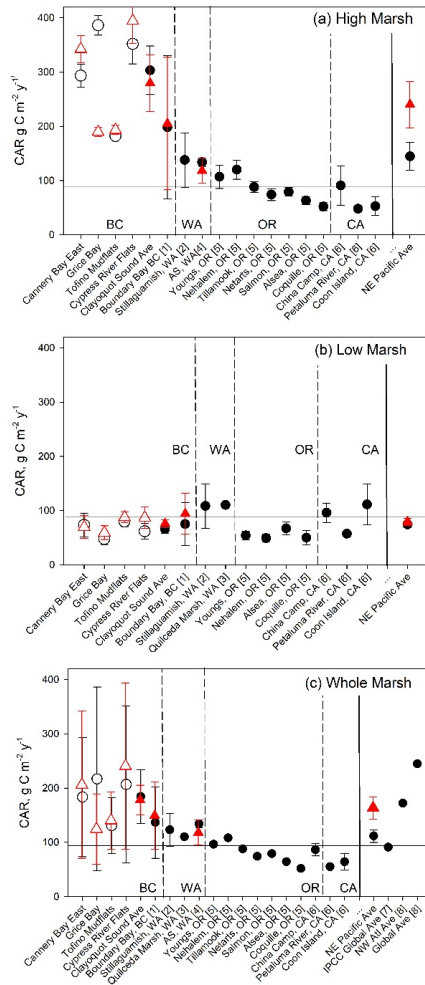
Figure 7. Comparison of Clayoquot Sound CARs with other salt marshes with ^{210}\text{Pb} dating, for whole core (black circles) and 30- 485 year (red triangle) estimates. Individual Clayoquot Sound marshes are indicated with open symbols followed by a regional mean ( \pm SE). Additional site data taken from: [1] Boundary Bay, BC, Canada (Gailis et al., 2021); [2] Stillaguamish, WA, USA (Pope and
