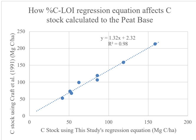
665 Figure A4. Comparison of C stocks (Mg C/ha) estimated using the Craft et al. (1991) equation versus C stocks estimated using this study's empirical relationship for southern BC, for 8 cores from our study region. Comparison suggests that using the Craft et al. (1991) relationship would produce C stocks that are ~32% greater than our estimates. This difference, while substantial, would not account for global C stocks that are 3 times larger than those found in Clayoquot Sound salt marshes.
