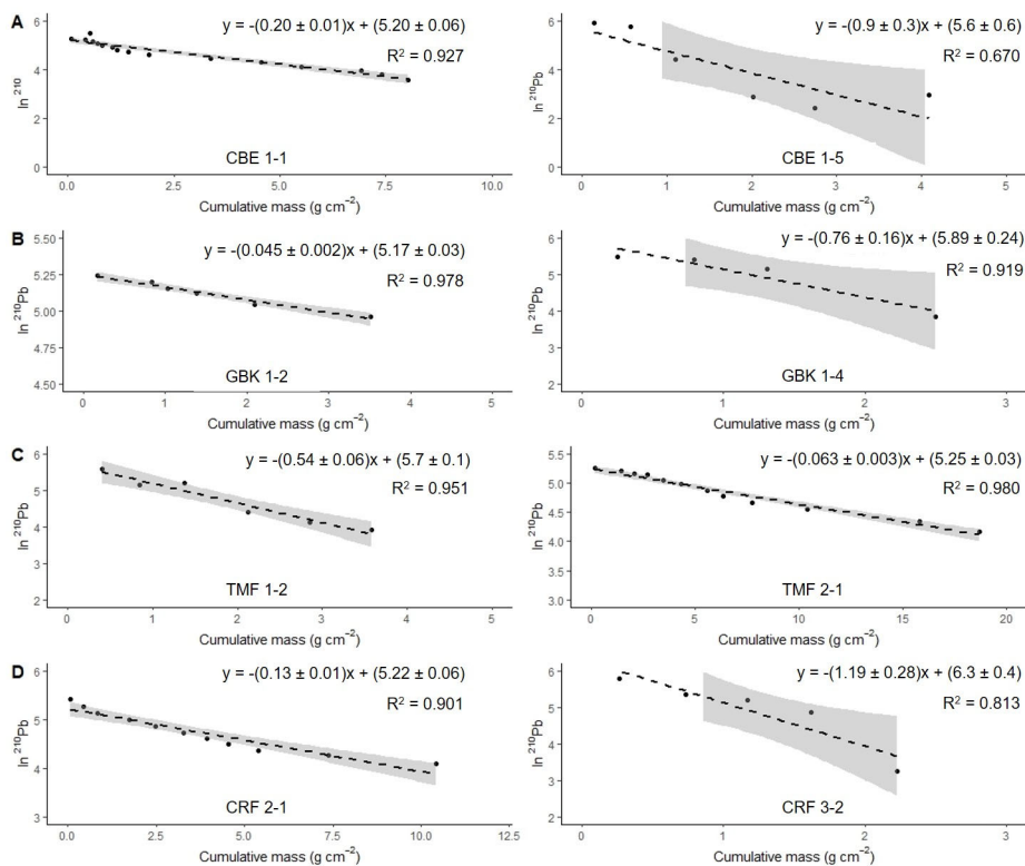
370 Figure 6. Natural log of Excess ^{210}\text{Pb} activity versus cumulative mass from the surface. The equation in each graph shows the results from the regression analyses used for the calculation of the mean accumulation rate ( \text{g cm}^{-2} \text{y}^{-1} ) using the CF:CS model. Grey shaded area represents 95% confidence intervals.
