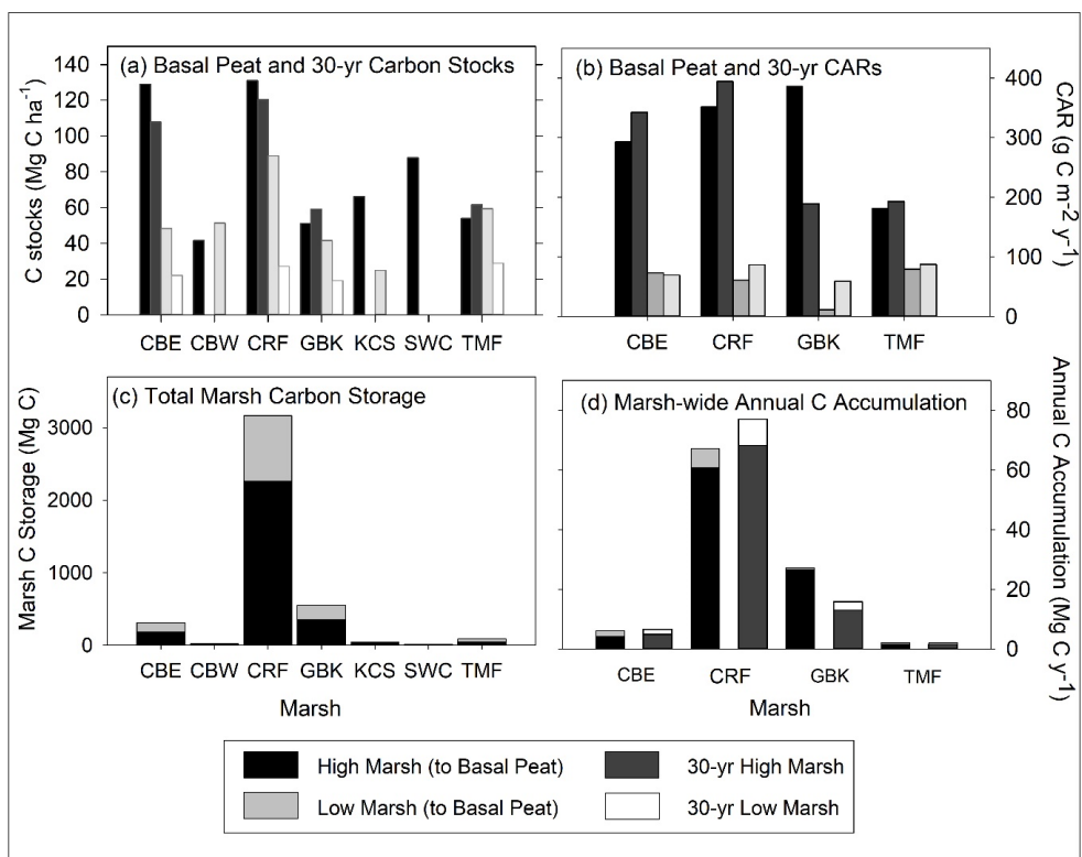
Figure 5. (a) High and low marsh carbon stocks ( \text{Mg C ha}^{-1} ) measured to the base of peat layer and for the last 30 years; (b) High and low marsh carbon accumulation rates (CARs, \text{g C m}^{-2} \text{y}^{-1} ) measured to the base of peat layer and for the last 30 years; (c) total marsh carbon ( \text{Mg C} ) estimate to the base of peat layer for high and low marsh zones of each marsh, and (d) marsh wide annual C accumulation ( \text{Mg C y}^{-1} ) estimated to the base of peat layer and for the last 30 years. Paired differences between high and low marsh CARs are statistically significant for CARs calculated to the base of peat layer ( t=4.283 , p\text{-value} = 0.0234 ) and for 30-yr CARs ( t=4.043 , p\text{-value} = 0.0272 ). (Statistical comparisons of C stocks are in Fig. 4).
