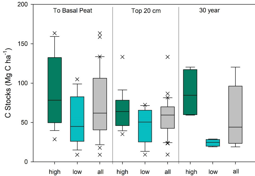
310 Figure 4. Carbon stock estimates for Clayoquot Sound for the high marsh zone (green), low marsh zone (blue), and combined (grey) for all cores. Estimates are made to the base of peat layer, for the surface 20 cm, and for the most recent 30 years of accretion. Note that 30-yr values are based on 4 cores each for high and low marshes (see Methods). Unpaired t-tests show statistically significant differences between the high and low marsh C stocks calculated to the base of peat depth ( t = 2.91 , p -value = 0.0065), 20-cm C stocks 315 ( t = 2.20 , p -value = 0.036) and 30-year C stocks ( t = 3.95 , p -value = 0.0074).
