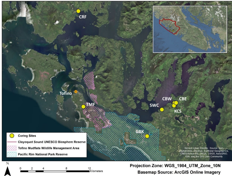
Figure 1. Site locations. Cypress River Flats (CRF), Cannery Bay East (CBE), Cannery Bay West (CBW), Kennedy Cove South (KCS), Shipwreck Cove (SWC), Grice Bay at Kootowis Creek (GBK), and Tofino Mudflats (TMF). Pacific Rim National Park and Reserve (blue crosshatching) covers the southern portion of the map and the Tofino Mudflats Wildlife Management Area (pink crosshatching) covers portions of the southwestern area. The study region lies within the Clayoquot Sound UNESCO Biosphere Reserve, British Columbia, Canada (inset, outlined).
