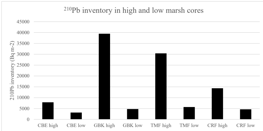
670 Figure A5. ^{210}\text{Pb} inventory (Bq m -2 ) in high and low marsh cores.
