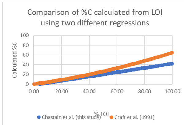
Figure A3. Comparison of %OC calculation using the empirical regression determined for our study area (blue) and the model of Craft et al. (1991) (orange).
