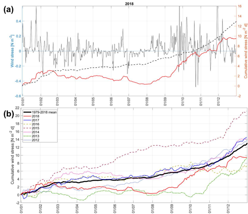
Figure 8. (a) Time series of along-coast (NNE–SSW) component of wind stress \tau_{NNE} and cumulative wind stress in 2018 (6h moving average is shown). (b) Cumulative wind stress for each year in 2012–2018. Average cumulative wind stress curve for 1979–2018 is shown in both panels. Data were extracted from the ERA5 grid point outside the gulf (see location in Fig. 1).
