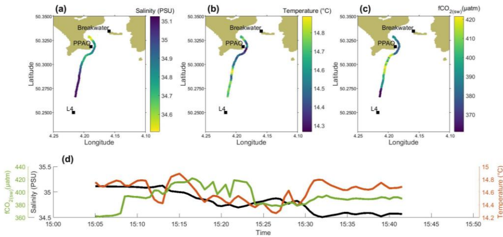
665 Figure 4: Example of a low water transect (transect mid-point = LW+0.5 hrs). Surface measurements of salinity, temperature and fCO 2 represented spatially (a to c) and as a time series (d) from station L4 toward the coast. Data were collected onboard RV Plymouth Quest on 7th July 2016 (filled circles, data every 30 sec).
