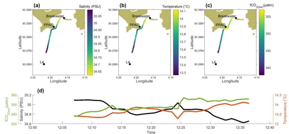
670 Figure 5: Example of a flooding tide transect (transect mid-point = LW+3.5 hrs). Surface measurements of salinity, temperature and fCO 2 represented spatially (a to c) and as a time series (d) from station L4 toward the coast. Data were collected onboard RV Plymouth Quest on 15th June 2016, (filled circles, data every 30 sec).
