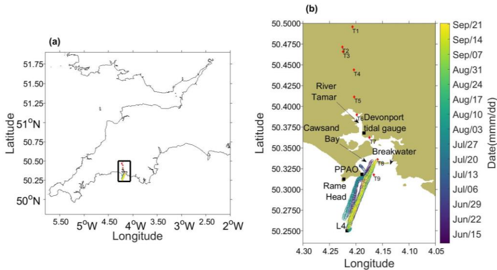
650 Figure 1: (a) Map of the Southwest of the England Western Channel Observatory (WCO) and study area (black rectangle). (b) Breakwater to L4 transects for the 15 transects made with the RV Plymouth Quest (coloured circles). Ship tracks are coloured by date between 10 th June and 21 st September 2016. The River Tamar, Devonport tidal gauge station, Plymouth Breakwater, Cawsand Bay, PPAO, Rame Head and Station L4 are marked. Transect sites T1-T9 are shown as red diamonds.
