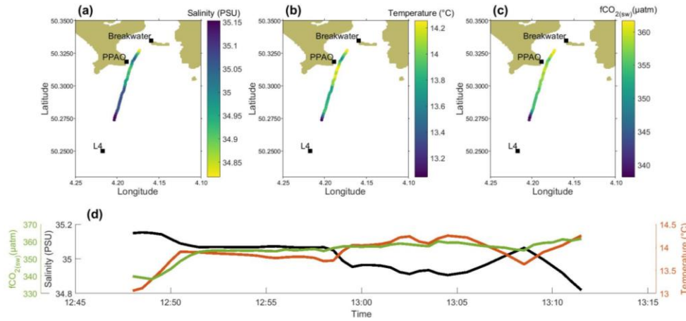
680 Figure 7: Example of an ebbing tide transect (transect mid-point = LW+8.75 hrs). Surface measurements of salinity, temperature and f\text{CO}_2 represented spatially (a–c) and as a time series (d) from station L4 toward the coast. Data were collected onboard RV Plymouth Quest on 10th June 2016, (filled circles, data every 30 sec).
