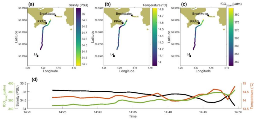
675 Figure 6: Example of a high water transect (transect mid-point = LW+6 hrs). Surface measurements of salinity, temperature and f\text{CO}_2 represented spatially (a–c) and as a time series (d) from station L4 toward the coast. Data were collected onboard RV Plymouth Quest on 30th June 2016, (filled circles, data every 30 sec).
