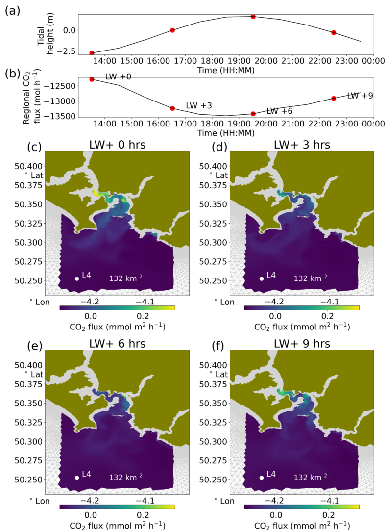
695 Figure 11: Modelled impact of a full tidal cycle (a) on tidal height (b) on air-sea CO 2 flux in the coastal zone (hourly calculations, negative fluxes are into the ocean) on 7 th July 2016 with a fixed wind speed of 5.3ms -1 . The total integrated air-sea CO 2 flux within the modelled domain (c-f). Spatial variation in flux at four different stages of the 12 hour tidal cycle is shown: LW+0 hr (c). LW+3 hr (d), LW+6 hr (e). LW+9 hr (f). The red dots in (a) and (b) correspond to panels c-f.
