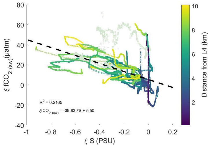
Figure 8: Scatter plot of \Delta S versus \Delta fCO_2 , difference of data from transects between Plymouth Breakwater and station L4 between 10th June and 21st September 2016. Data are coloured by their distance from station L4, the dashed black line is the best fit for the data. The data for 7th July is shown in light grey.
