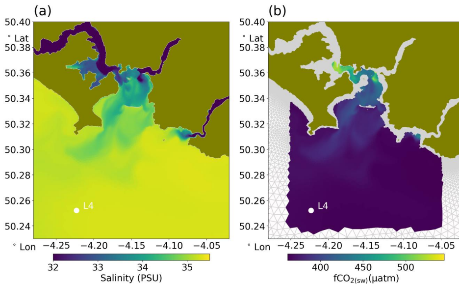
690 Figure 10: (a) Model surface salinity field on 7th July at the midpoint of the observational transect. Note that the range of the colourbar was restricted to better depict salinity in the lower estuary and thus salinity in the upper estuaries is beyond the range of the colourbar. (b) derived \xi fCO_2 using determined \xi S and \xi fCO_2 relationship.
