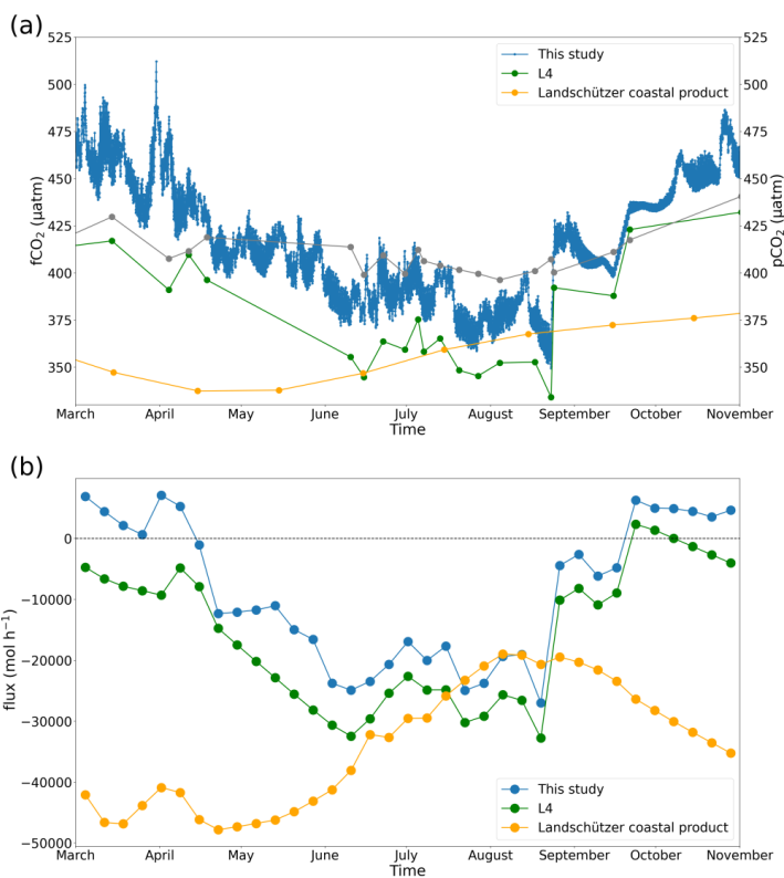
Figure 12: (a) f\text{CO}_2 and p\text{CO}_2 values used to calculate regional \text{CO}_2 flux over the domain ( 128 \text{ km}^2 , approximately same as in above figures). Measurements of f\text{CO}_2 made by RV Plymouth Quest on station at L4 (L4, green dots). p\text{CO}_2 ( \text{atm} ) measured by Plymouth Quest on station at L4 (grey squares). The results of this study, hourly average f\text{CO}_2 across the valid model domain used for long term flux calculations (this study, blue dots). The standard combined uncertainty in the data from this study is indicated by the shaded background in light blue. The monthly Landschützer p\text{CO}_2 data (Landschützer coastal product, orange dots) is from the closest valid node ( 50.125^\circ\text{N} , 4.125^\circ\text{W} ) in the Landschützer et al. (2020) coastal data product. (b) Regional \text{CO}_2 flux calculated using the three different \text{CO}_2 over the valid model domain used for long term flux calculations ( 128 \text{ km}^2 , approximately same as in above figures). All fluxes were calculated using average monthly wind speed from the L4 buoy and using interpolated p\text{CO}_2 ( \text{atm} ) measured by RV Plymouth Quest . For this study fluxes were calculated across the domain using model derived f\text{CO}_2 , temperature and salinity. The flux for the Landschützer and L4 measurements were calculated using temperature and salinity from the L4 buoy and scaled up to the equivalent area as this study. It is noted that the Landschützer node is outside of the model domain (which has a lower boundary of 50.24^\circ\text{N} ) and that the fluxes are made with p\text{CO}_2 rather than f\text{CO}_2 . The vertical dashed lines indicate the dates of the first and last measurement transects.
