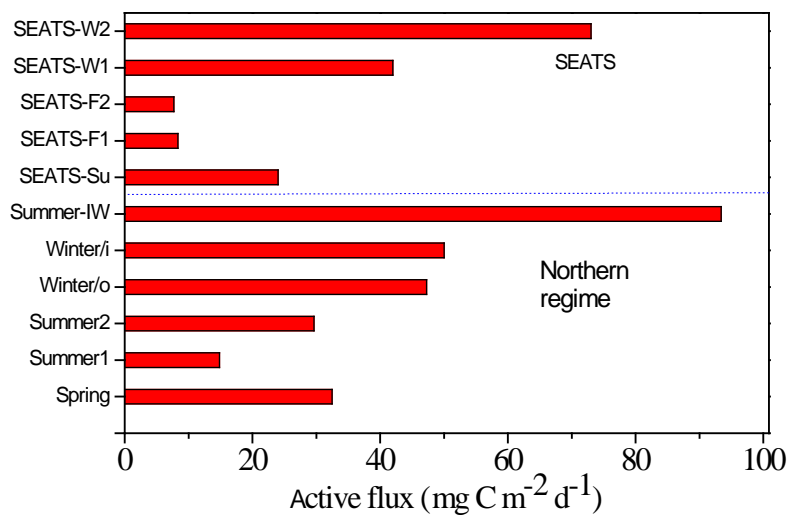
Figure 6 Comparisons between seasonal and spatial active carbon fluxes in the NSCS. The active fluxes were geographically grouped as the central basin represented by the SEATS station and the northern regime for other sampling locations. The SEATS active fluxes were estimated using the empirical relationship between active fluxes and inventories of Chl- a except for SEATS-F1 and F2 (fall season), which were derived from experimental data. The data of the northern regime were all experimental data, except for the Winter/o (outside the eddy) datum derived from the empirical relationship between active fluxes and Chl- a inventories. Winter/i (inside the eddy); Summer-IW (internal waves); SEATS-Su (summer); SEATS-W (winter); SEATS-F (fall).
