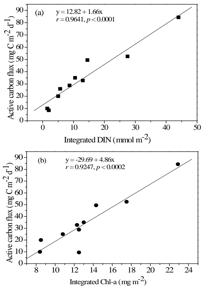
Figure 5 Empirical relationship between active carbon fluxes and DIN inventories in the euphotic zone (a) and between active carbon fluxes and Chl- a inventories in the euphotic zone (b). The statistic correlations were established from collected data in allvarious expeditions.
