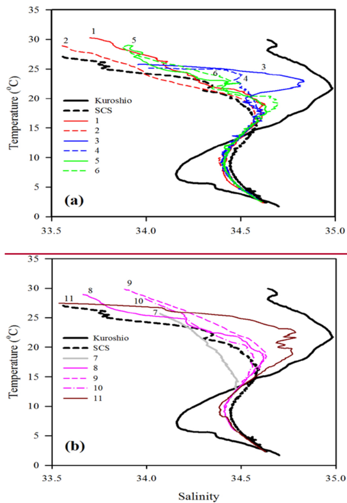
325 Figure 3 T–S plots for comparing water-column characteristics among stations 1–6 (a) and stations 7–11 (b). Kuroshio and SCS indicated denote the typical T–S features of Kuroshio and South China Sea waters, respectively. The Kuroshio and SCS waters are represent typical waters collected from the West Philippine Sea and central SCS central basin, respectively.
