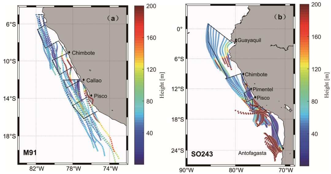
Figure 6. Air mass backward trajectories of cruise M91(a) and SO243 (b), with colorbar indicating the height above sea level. Note that both scales are capped at 200 m to ensure readability of the plots, despite that some values exceed the upper threshold.
