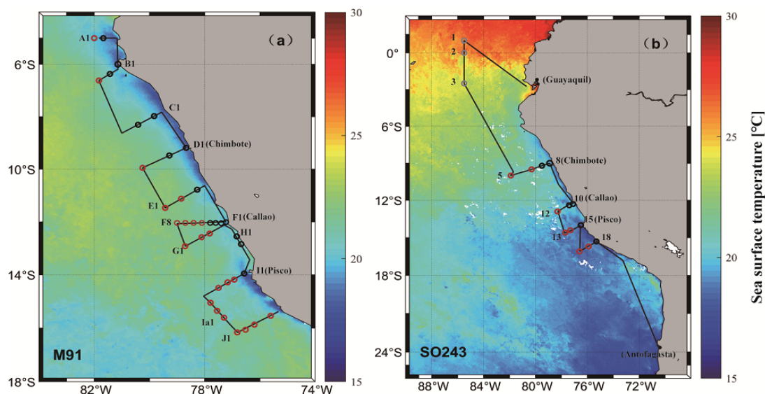
40 Figure1: Cruise tracks of M91 (a) and SO243 (b) plotted on top of monthly mean SST detected by the Moderate Resolution Imaging Spectroradiometer (MODIS) instrument on board the Aqua satellite. Red circles indicate offshore stations, and black circles indicate coastal stations in both panels. Grey circles in panel b indicate equatorial stations. Note that no CTD cast was performed at stations 4 and 9 during cruise SO243.
