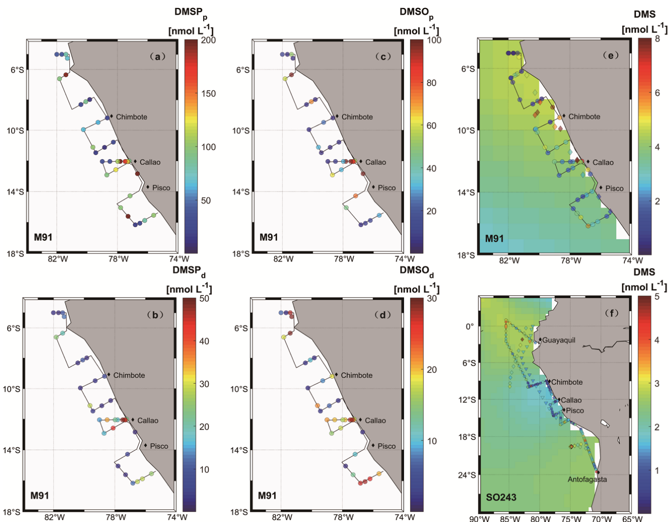
Figure 3. Surface seawater measurements of sulfur compounds are shown in panels a–f (circles) for DMSP p (M91), DMSP d (M91), DMSO p (M91), DMSO d (M91), DMS (M91) and DMS (SO243), respectively. Monthly (December and October) surface DMS concentrations from the Lana et al. (2011) climatology are colour-coded in the background in e and f, respectively. Diamonds in panel e, as well as diamonds and triangles in panel f, are recorded DMS concentrations in adjacent waters retrieved from the PMEL database for June–July 1982 (Andreae, 1985), October–November 2007 (unpublished DMS data) and October–November 2008 (Hind et al., 2011), respectively. Note that to ensure readability of the plots, the scale in panel e is capped at 8 nmol L -1 with a few values exceeding the upper threshold, and DMS data retrieved from the PMEL database were averaged every ten samples.
