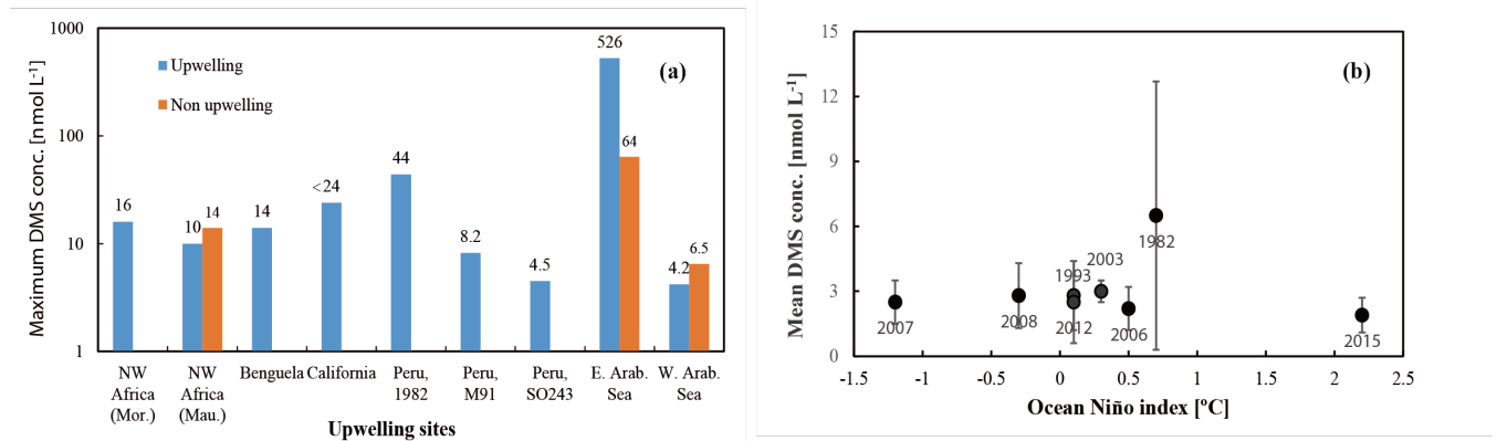
Figure 5. (a): Maximum DMS concentrations measured in various upwelling regions worldwide. Mor. stands for Morocco and Mau. stands for Mauritania. (b): Mean and standard deviation of DMS concentrations for each cruise in the ETSP. Note that the value from 2003 only includes the data east of 95 °W.
