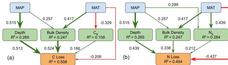
Figure 5. Diagram of proposed pathways for the effects of MAP and MAT on C (a) and N (b) loss. Non-climate variables regard the organic layer. Each variable node is labeled with the R^2 from simple or multiple regression using explanatory variables represented by all incoming arrows. Arrows are labeled by and sized in proportion to the magnitude of their standardized regression coefficients and are significant. Green arrows represent positive relationships while red represent negative relationships. Omitted for simplicity are direct correlations between bulk density to C_R ( p = 0.010 , r = 0.356 ) and depth to N_R ( p = 0.010 , r = -0.363 ).
