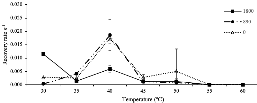
Fig. 4: Recovery rate s -1 of F v /F m after the RLC for low irradiance experiments. Recovery rates were plotted against experimental temperatures at irradiances of (1800 μmol photons m -2 s -1 (close square), 890 μmol photons m -2 s -1 (close circle) and 0 photons m -2 s -1 (open triangles)) and temperatures (30, 35, 40, 45, 50, 55 and 60 °C). In this recovery analysis, samples of 30 °C and 35 °C were analyzed without replicates; thus, no error bar was obtained.
