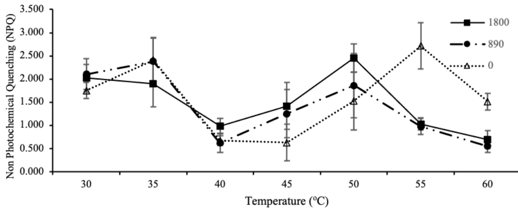
Fig. 3: The NPQ of samples at each irradiance level (1800 photons m -2 s -1 (close square), 890 photons m -2 s -1 (close circle) and 0 photons m -2 s -1 (close triangles)) and temperatures (30, 35, 40, 45, 50, 55 and 60 °C). NPQ was obtained at the end of the RLCs with actinic irradiance of 1554 μmol photons m -2 s -1 . Values are means ± SD ( n = 3).
