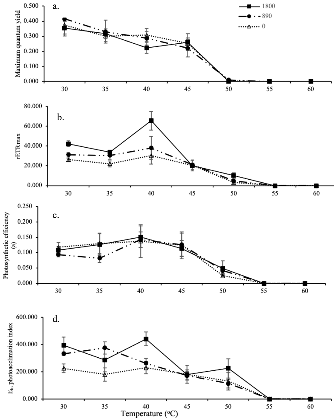
Fig. 2: Derived photosynthetic parameters of RLC. Parameters were plotted against experimental temperatures (30, 35, 40, 45, 50, 55 and 60 °C) at irradiances of 1800 \mu\text{mol photons m}^{-2} \text{s}^{-1} (close square), 890 \mu\text{mol photons m}^{-2} \text{s}^{-1} (close circle) and 0 \mu\text{mol photons m}^{-2} \text{s}^{-1} (open triangles). a) Maximum quantum yield, b) Photosynthetic efficiency ( \alpha ), c) rETRmax and d) Photoacclimation index, ( E_k ). Values are means \pm SD ( n = 3 ).
