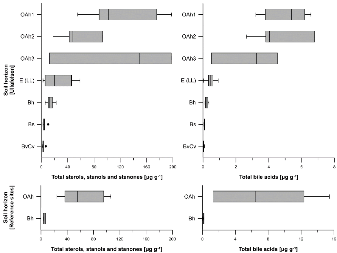
690 Figure 5: Box plots illustrating the total steroid (sterols, stanols, stanones and bile acids) contents (in µg g -1 dry matter) of the investigated soil profiles from the prehistorical encampment site of Ullafelsen and reference sites in the Fotsch Valley, Stubai Alps, Austria, categorized by the soil horizons OAh1 (n=6), OAh2 (n=4), OAh3 (n=3), E (LL) (n=8), Bh (n=6), Bs (n=5) and BvCv (n=5).
