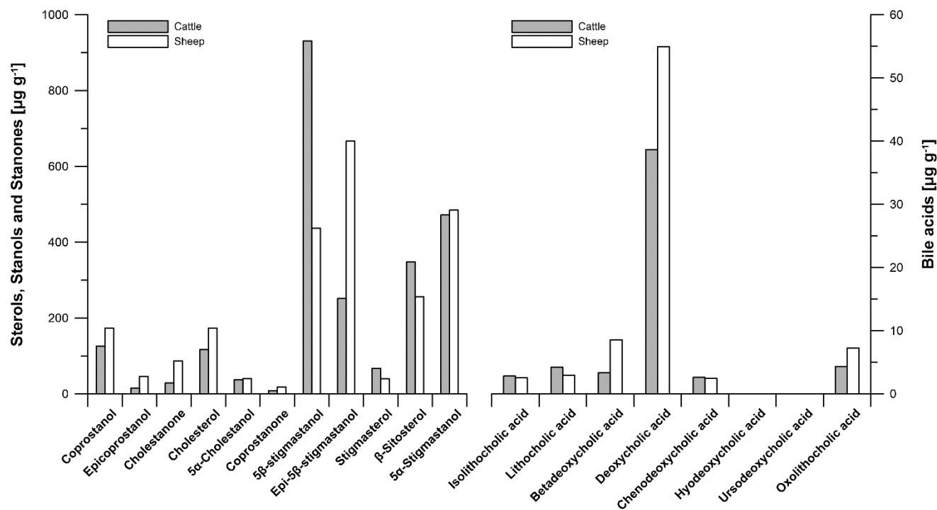
Figure 4: Biomarker patterns of modern faeces from predominating livestock animals at the prehistorical encampment site of Ullafelsen in the Fotsch Valley, Stubai Alps, Austria and surroundings. Steroid (sterols, stanols, stanones and bile acids) contents of cattle and sheep faeces are given in \mu\text{g g}^{-1} dry matter.
