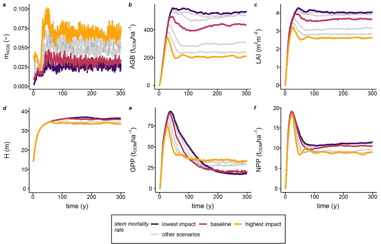
300 Figure 3: Simulation results of the (a) biomass loss rate ( m_{AGB} ), (b) aboveground biomass (AGB), (c) leaf area index (LAI), (d) mean forest height (H), (e) gross primary production (GPP), and (f) net primary production (NPP) of terra firme forest stands under different stem mortality intensities. Grey lines indicate the entire set of scenarios under varying stem mortality rates (eq. 1) (ODM: organic dry matter; for further details see Tab. 1, Fig. S2 and Fig. S3).
