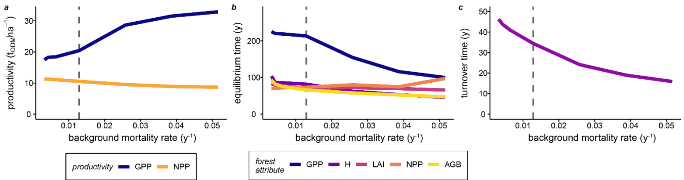
315 Figure 4: Influence of stem mortality levels in simulated terra firme forests on (a) mature forests’ mean GPP and mean NPP (averages over simulation years 250 – 300), (b) the time until the forest attributes reached equilibrium states, and (c) the mean biomass turnover times, represented as the reciprocal values of the biomass loss rate (cf. eq. 5; averages over years 0–300). Dashed lines indicate the baseline scenario (GPP: gross primary production, NPP: net primary production, H: forest height, LAI: leaf area index, AGB: aboveground biomass, ODM: organic dry matter).
