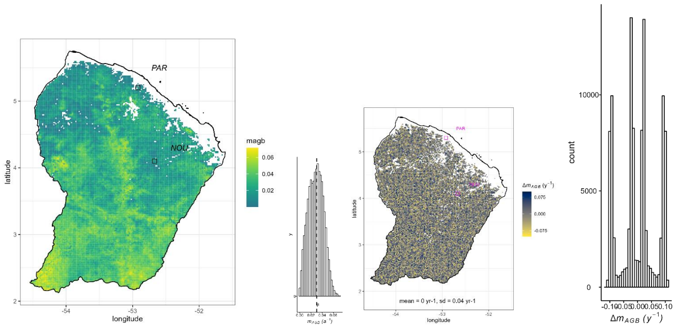
380 Figure 7: (a) Map of biomass loss for terra firme forests in French Guiana (~ 2 km resolution) and (b) its histogram. The dashed line in b) indicates the estimated country-wide mean (3.10% with a standard deviation of 1.92%). The black squares in the map show the locations of forest plots at Paracou (PAR) and Nourage (NOU), from which census-data was used to compare estimated and field-based biomass loss values. (c) The census data originate from Brienen et al., (2015). (d) Sensitivity analysis for the mapped biomass loss rates of terra firme forests in French Guiana (cf. Fig. 7.a) and (e) its histogram. The values for the input maps of leaf area index (LAI) and forest height were randomly sampled using a uniform distribution ranging between \pm 30\% from their original values (cf. Fig. S4). \Delta m_{AGB} represents the variation in biomass loss rates given this variation in the input variables. For further results about the uncertainty analysis performed, see Fig. S7, Fig. S8, Fig S9, Fig. S10, Fig. S11, and Fig. S14. Note that there are accompanying uncertainty products to the remote sensing products that could be considered to estimate error propagation. 385
