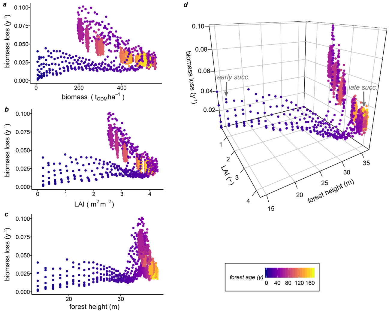
330 Figure 5: Dependence of biomass loss rates from single attributes (a) biomass, (b) LAI, (c) forest height versus (d) the multiple forest attributes, LAI and forest height, of simulated forest states, including all stem mortality scenarios. Each dot represents a terra firme forest stand with a unique forest structure (i.e., tree size distribution and functional species composition). All simulated years are included in the analyses. The colours of the dots show the mean forest ages characterising the successional states (ODM: organic dry matter).
