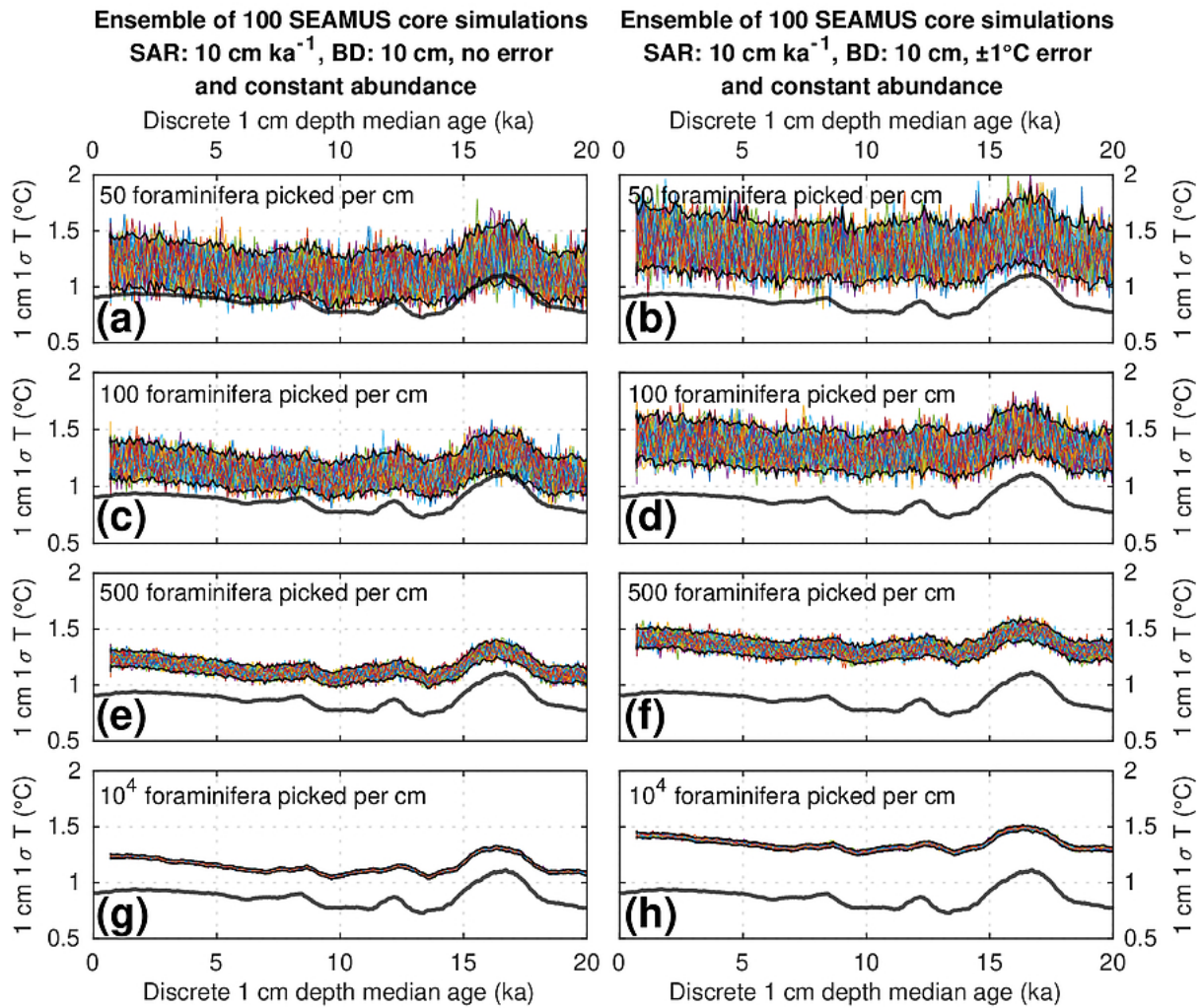
Figure 3. Simulated downcore, discrete 1 cm depth 1\sigma SST values of simulated single foraminifera from various 10 \text{ cm ka}^{-1} SAR scenarios with 10 cm BD, each with 100 ensembles of SEAMUS runs. In each panel, each ensemble is shown using a coloured line. The solid black lines represent the 95% interval of the ensemble runs at each discrete 1 cm depth. Also shown for reference as a thick grey line is the 1000 year (12000 month) moving 1\sigma of the 1.5-7 year filtered monthly SST data (as also shown in Fig. 1c.) The left panels (a, c, e and g) show the output of scenarios with 50, 100, 500 and 10^4 randomly picked foraminifera per discrete 1 cm depth, all with constant species abundance and no assumed analytical error. The right panels (b, d, f and h) show the output of scenarios with 50, 100, 500 and 10^4 randomly picked foraminifera per discrete 1 cm depth, all with constant species abundance and an assumed analytical error of \pm 1^\circ\text{C} in SST.
