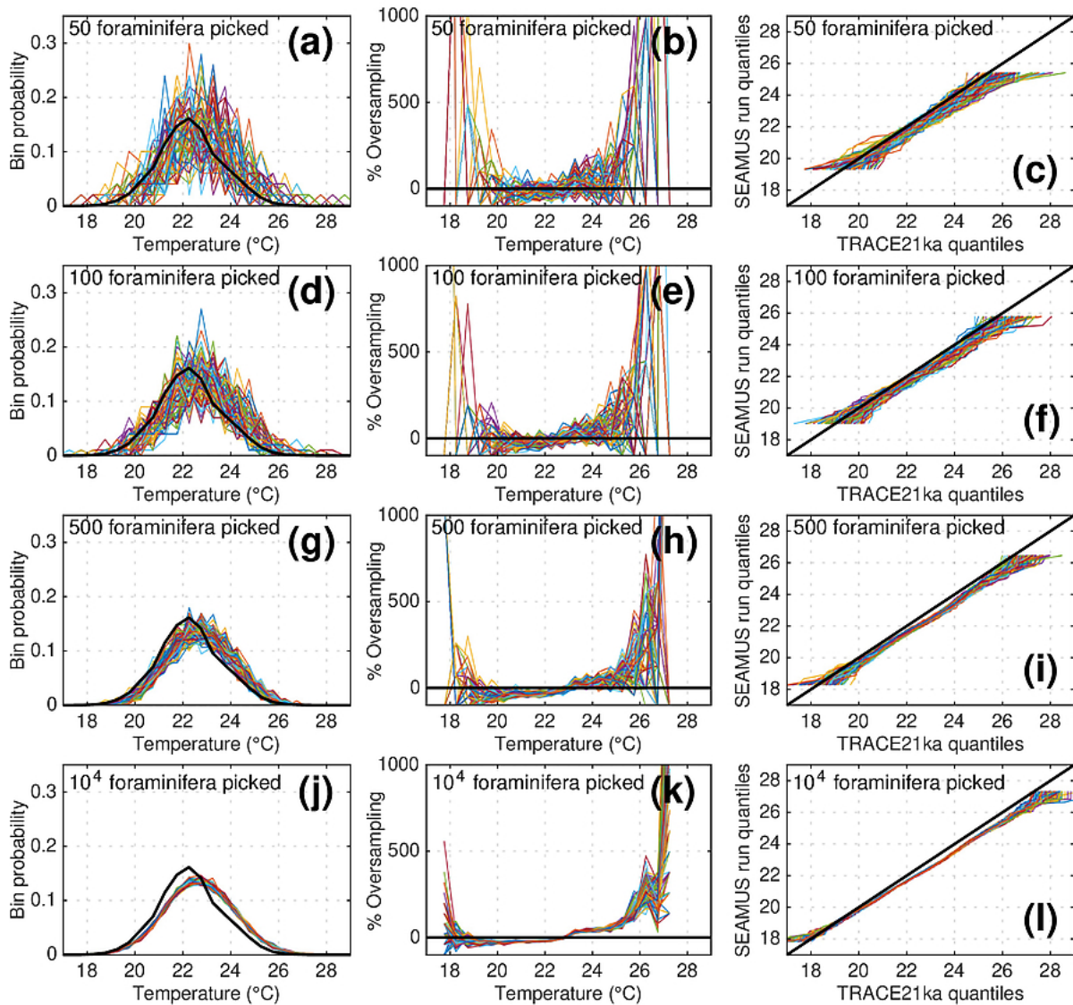
Figure 8. Simulated single foraminifera SST distributions from 100 ensembles of SEAMUS runs, with SAR of 10 cm ka -1 , BD of 10 cm, ±1 °C analytical error and dynamic abundance (following Fig. 2a). In each ensemble, the single foraminifera SST distribution from a single discrete depth with a simulated median age of 17.5 ka is shown, and compared to the TRACE-21ka SST distribution for the 18 ka to 17 ka period. The left panels (a, d, g and j) show the 100 SEAMUS ensembles as coloured lines in the case of 50, 100, 500 and 10 4 randomly picked foraminifera, with the TRACE-21ka SST distribution is shown as a black line. The middle panels (b, e, h and k) show the the rate of over/undersampling for each of the 100 SEAMUS ensembles (coloured lines) relative to the TRACE-21ka SST distribution (black line) in the case of 50, 100, 500 and 10 4 randomly picked foraminifera. The right panels (c, f, i and l) show Q-Q plots of the 100 SEAMUS ensemble quantiles vs the TRACE-21ka quantiles as coloured lines in the case of 50, 100, 500 and 10 4 randomly picked foraminifera, with a perfect 1:1 correspondence to TRACE-21ka shown for reference as a black line.
