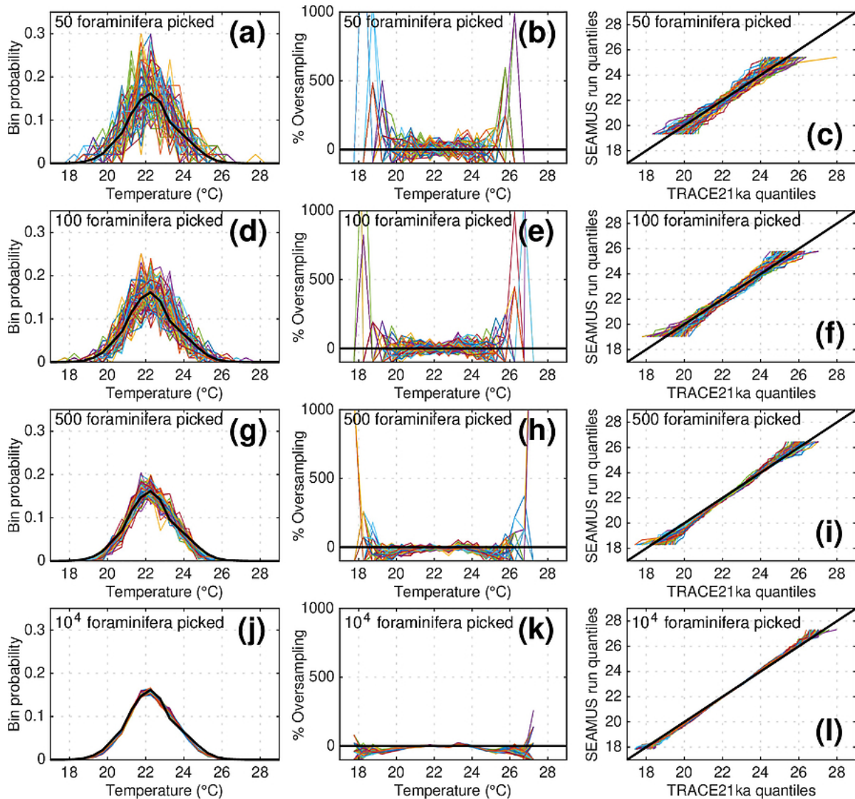
460 Figure 5. Simulated single foraminifera SST distributions from 100 ensembles of SEAMUS runs, with SAR of 10 cm ka -1 , BD of 10 cm, no analytical error and constant abundance. In each ensemble, the single foraminifera SST distribution from a single discrete depth with a simulated median age of 17.5 ka is shown, and compared to the TRACE-21ka SST distribution for the 18 ka to 17 ka period. The left panels (a, d, g and j) show the 100 SEAMUS ensembles as coloured lines in the case of 50, 465 100, 500 and 10 4 randomly picked foraminifera, with the TRACE-21ka SST distribution is shown as a black line. The middle panels (b, e, h and k) show the the rate of over/undersampling for each of the 100 SEAMUS ensembles (coloured lines) relative to the TRACE-21ka SST distribution (black line) in the case of 50, 100, 500 and 10 4 randomly picked foraminifera. The right panels (c, f, i and l) show Q-Q plots of the 100 SEAMUS ensemble quantiles vs the TRACE-21ka quantiles as coloured lines in the case of 50, 100, 500 and 10 4 randomly picked foraminifera, with a perfect 1:1 correspondence to TRACE-21ka shown for reference as a black line. 470
