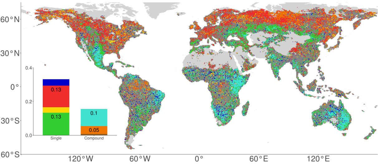
b) Hydro-meteorological hazards during SIF minima
