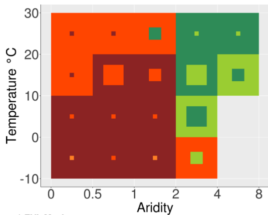
c) EVI, Maximum
