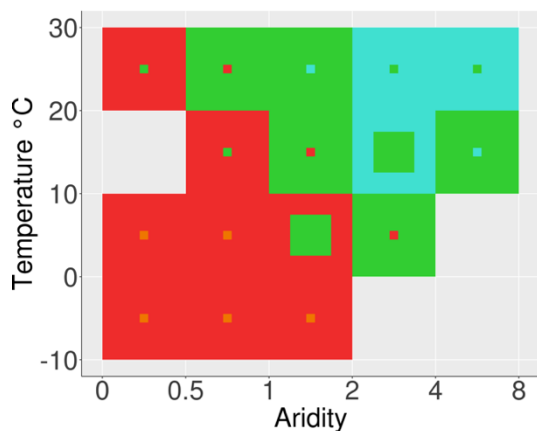
e) Hazards, Maximum
