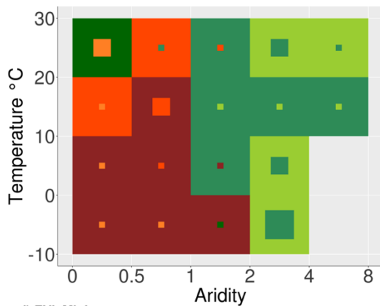
d) EVI, Minimum
