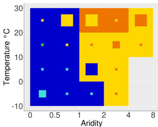
f) Hazards, Minimum
