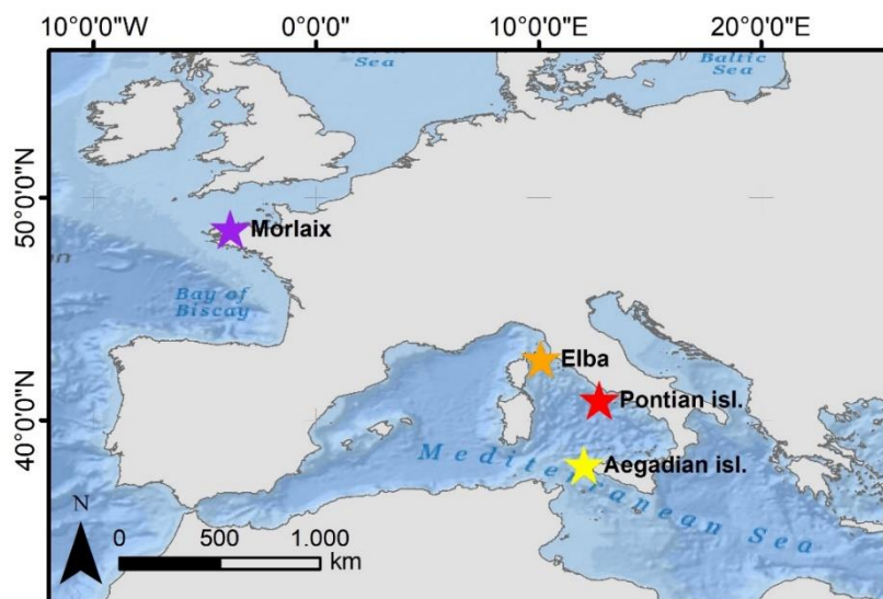
120 Figure 1: Map showing the distribution of sampling sites where Lithothamnion corallioides samples were collected: Morlaix Bay (48°34'42"N, 3°49'36"W); Aegadian Islands (37°97'36"N, 12°14'12"E); Elba (42°44'56.4"N, 10°07'08.4"E) and Pontian Islands (40°54'N, 12°45'E). Service layer credits: Source Esri, GEBCO, NOAA, National Geographic, Garmin, geonames.org and other contributors.
