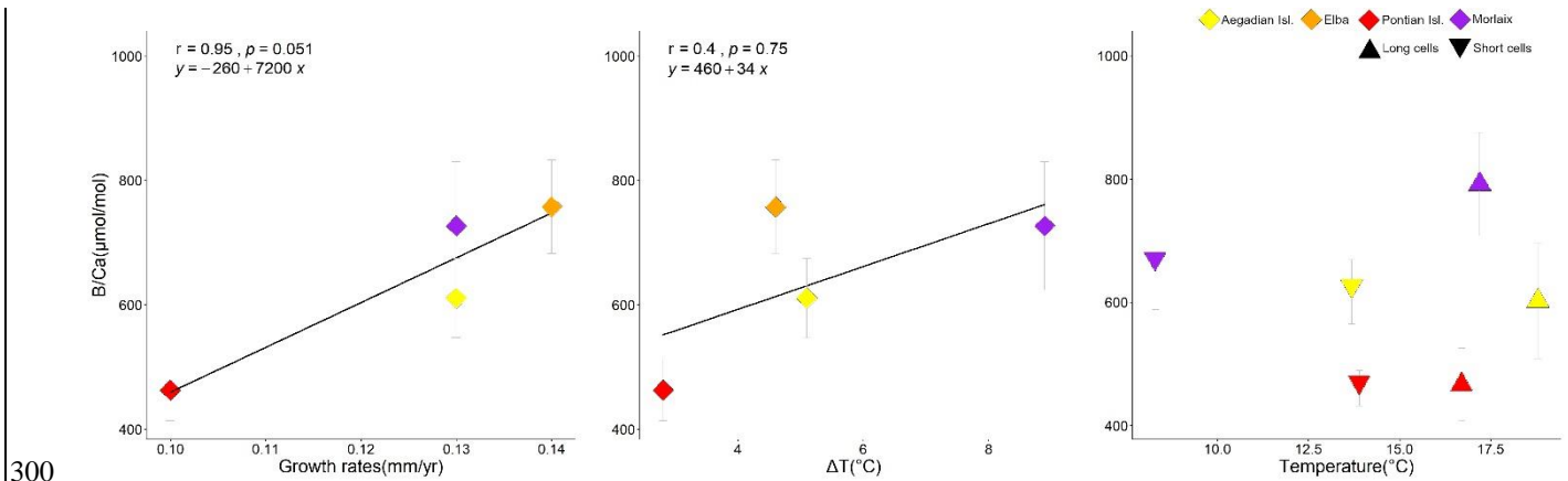
Figure 11: Correlation plots of growth rates and seawater temperature with B/Ca in L. corallioides samples analysed in this study. Spearman's coefficient r , the p -value and the line equation are given. Temperature variations ( \Delta T ) correspond to the differences between the maximum and minimum temperature registered over 11 years of monthly reanalysis (ORASS). The B/Ca means measured in long and short cells correspond respectively to the maximum and minimum temperature.
