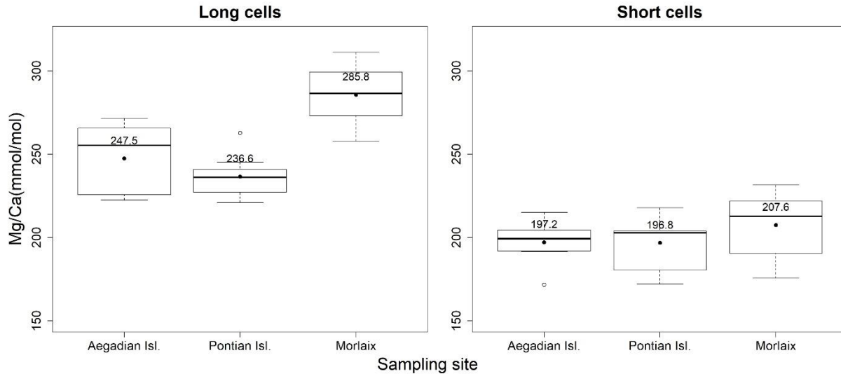
245 Figure 5: Box plots of the statistical tests performed to evaluate the differences of Mg/Ca in the long and short cells of L. corallioides collected in different sampling sites. The horizontal black lines indicate the median values. The black filled circles and the numbers inside the plot indicate the mean values.
