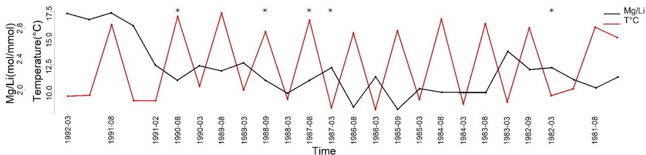
255 Figure 7: Mg/Li ratio of L. corallioides collected in Morlaix Bay. Note the lack of cyclic variations in Mg/Li results. In the timeline, the coldest and the warmest months have been reported. Mg/Li in the missing bands (asterisks) have been calculated as the means of the values measured in warm and cold periods. Monthly means of seawater temperature have been extracted by ORAS5 reanalysis.
