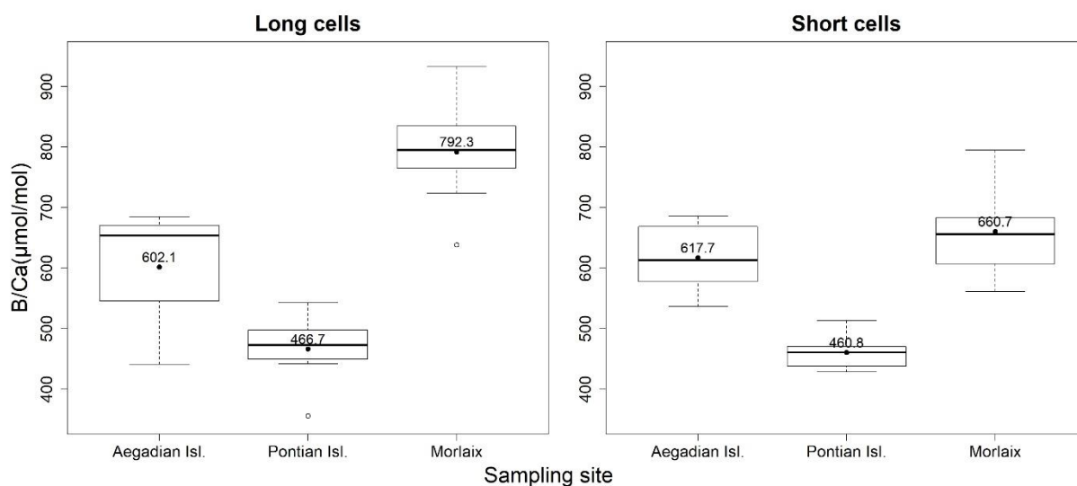
290 Figure 10: Box plots of the statistical tests performed to evaluate the differences of B/Ca in the long and short cells of L. corallioides collected in different sampling sites. The horizontal black lines indicate the median values. The black filled circles and the numbers inside the plot indicate the mean values.
