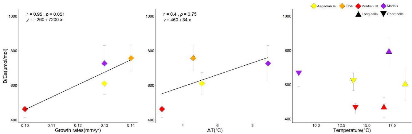
305 Figure 11: Correlation plots of growth rates and seawater temperature with B/Ca in L. corallioides samples analysed in this study. Spearman's coefficient r , the p -value and the line equation are given. Temperature variations ( \Delta T ) correspond to the differences between the maximum and minimum temperature registered over 11 years of monthly reanalysis (ORAS5). The B/Ca means measured in long and short cells correspond respectively to the maximum and minimum temperature.
