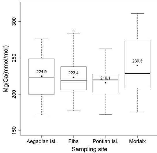
235 Figure 4: Box plot of the statistical tests performed to evaluate the differences of Mg/Ca in L. corallioides collected in different sampling sites. The horizontal black lines indicate the median values. The black filled circles and the numbers inside the plot indicate the mean values.
