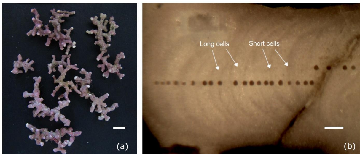
160 Figure 2: (a) Thalli of Lithothamnion corallioides collected in Morlaix (scale bar = 5 mm). (b) Longitudinal section through the L. corallioides branch sampled in Morlaix showing the LA-ICP-MS transects targeting each growth bands (scale bar = 200\text{ }\mu\text{m} ).
