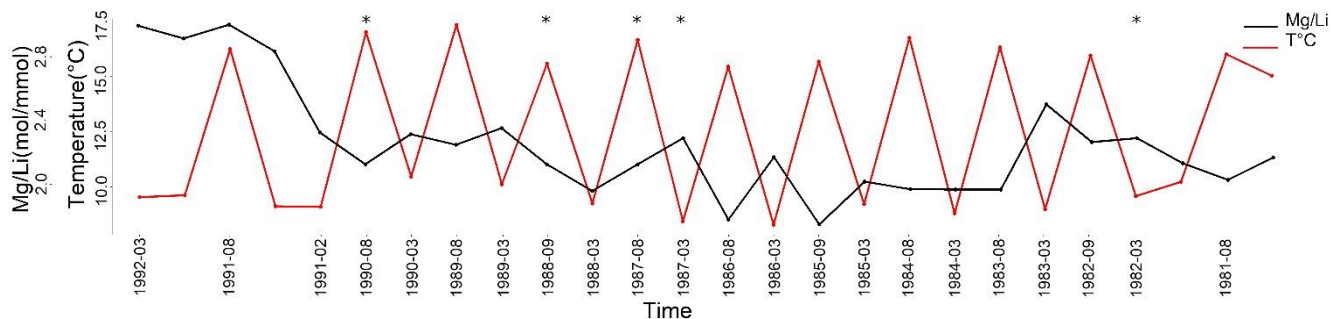
Figure 7: Mg/Li ratio of L. corallioides collected in Morlaix Bay. Note the lack of cyclic variations in Mg/Li results. In the timeline, the coldest and the warmest months have been reported. Mg/Li in the missing bands (asterisks) have been calculated as the means of the values measured in warm and cold periods. Monthly means of seawater temperature have been extracted by ORASS reanalysis.
