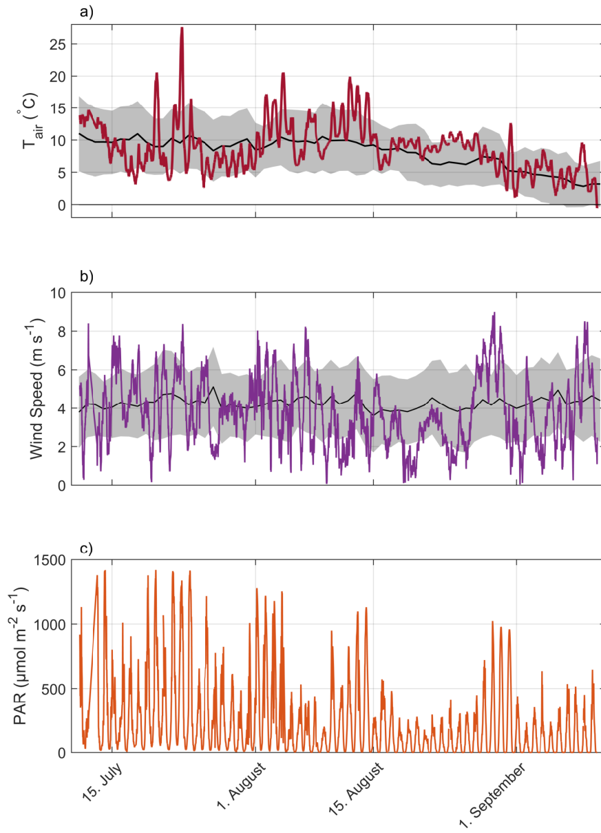
Figure A2. Timeline of observed meteorological conditions during the observation period with air temperature in 2 meters height (a), wind speed in 3 meters height (b) and photosynthetically active radiation (PAR) (c). Mean values and standard deviation of observations during the past 16 years are plotted as black lines and gray areas.
