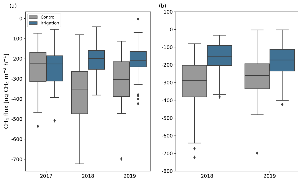
Figure 6. CH 4 fluxes measured by long-term (C1, C4, C6, C8, I2, I3, I4, I9) (a) and all (b) chamber points in May-September in different years. For comparison, the flux of the points located on the irrigated plot in 2018 and 2019 have been calculated already for 2017, even though the irrigation setup was established only in 2018. The boxes show the quartiles of the dataset and the horizontal line inside the boxes is the median flux. Whiskers show the range of the data, except for the points that are determined to be outliers, which are shown with black diamonds.
