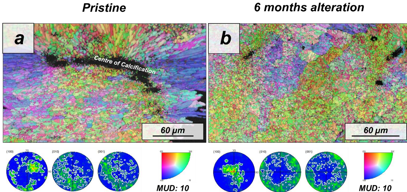
Figure 6. Colour-coded orientation maps with their corresponding pole figures derived from EBSD scans depicting the microstructure and texture of: (a) pristine and (b) altered coral, Porites sp., skeletons. Crystal co-orientation is given by the MUD value. No major changes can be observed between the pristine and the altered skeletal elements. However, we do not 295 discard that the alteration may have produced variations in the microstructure of Porites sp. that could not be detected by EBSD. The low co-orientation of the aragonite crystals in the pristine sample makes it difficult to see variations after alteration.
