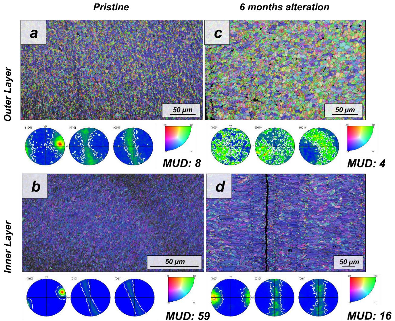
Figure 1. EBSD colour-coded orientation maps with their corresponding pole figures depicting aragonite microstructure and texture in: (a-b) pristine and (c-d) altered shells of the bivalve Arctica islandica . The strength of crystal co-orientation is given with the MUD value for the relevant EBSD scan, which is shown for each EBSD measurement. Even though that, at the applied hydrothermal alteration, new abiogenic calcite formation does not yet take place, the strong decrease in MUD values between the pristine and the altered samples indicates reorganization of the microstructure through new, abiogenic, aragonite formation.
