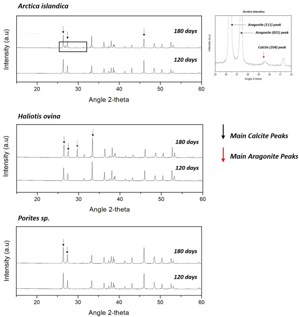
1130 Figure A2. X-ray diffractograms of the hydrothermally altered shells and skeletons of Arctica islandica , Haliotis ovina and Porites sp. Alteration was performed at 80°C in a Mg-rich, burial-mimicking fluid (100 mM NaCl + 10 mM MgCl 2 ) and lasted for 4 and 6 months.
