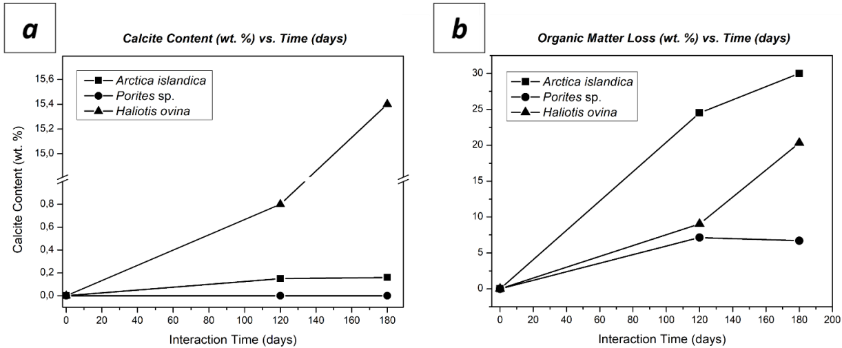
Figure 8. (a) Calcite content obtained from Rietveld analysis derived from XRD data and (b) organic matter loss measured with TGA with increasing alteration time. The influence of the individual aragonitic microstructure on both parameters is remarkable.
