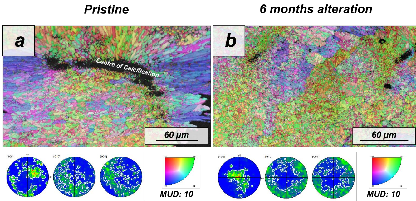
290 Figure 6. Colour-coded orientation maps with their corresponding pole figures derived from EBSD scans depicting the microstructure and texture of: (a) pristine and (b) altered coral, Porites sp., skeletons. Crystal co-orientation is given by the MUD value. No major changes can be observed between the pristine and the altered skeletal elements. However, we do not discard that the alteration may have produced variations in the microstructure of Porites sp. that could not be detected by EBSD. The low co-orientation of the aragonite crystals in the pristine sample makes it difficult to see variations after alteration.
