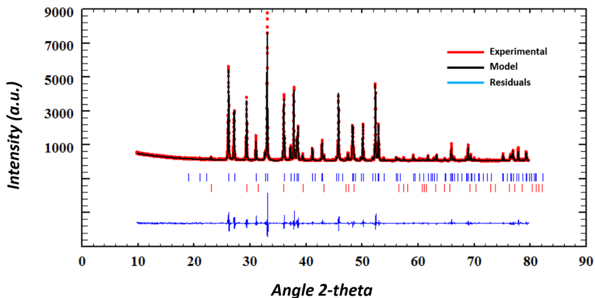
1200 Figure A14. Exemplary Rietveld refinement plot for an altered Haliotis ovina sample (6 months, 80 °C in Mg-rich fluid). Red dots: data points, black line: calculated XRD profile, bottom blue line: difference between observed and calculated data, blue vertical bars: positions of aragonite diffraction peaks, red vertical bars: position of calcite diffraction peaks.
