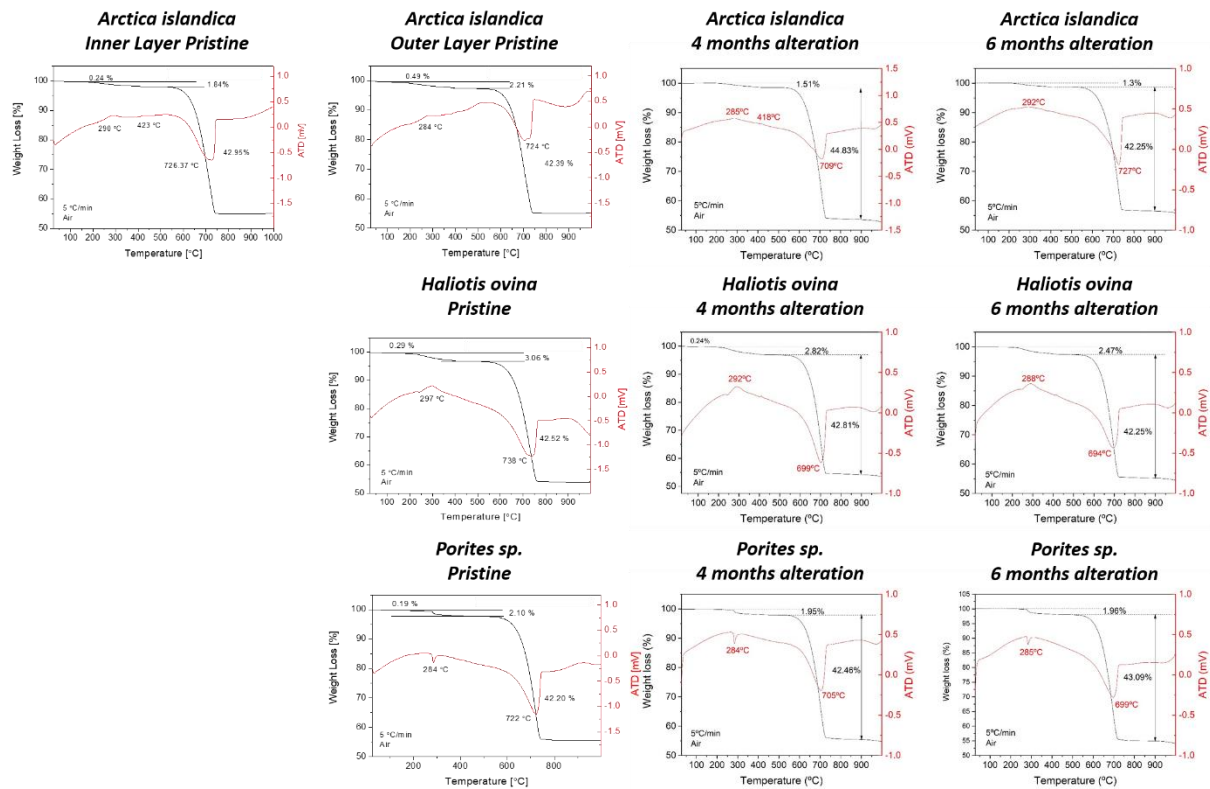
Figure A3. Thermogravimetric analysis data of pristine and altered hard tissues of Arctica islandica , Haliotis ovina and Porites sp. shells and skeletal elements. Alteration was performed at 80°C in a Mg-rich, burial-mimicking fluid (100 mM NaCl + 10 mM MgCl 2 ) and lasted for 4 and 6 months.
