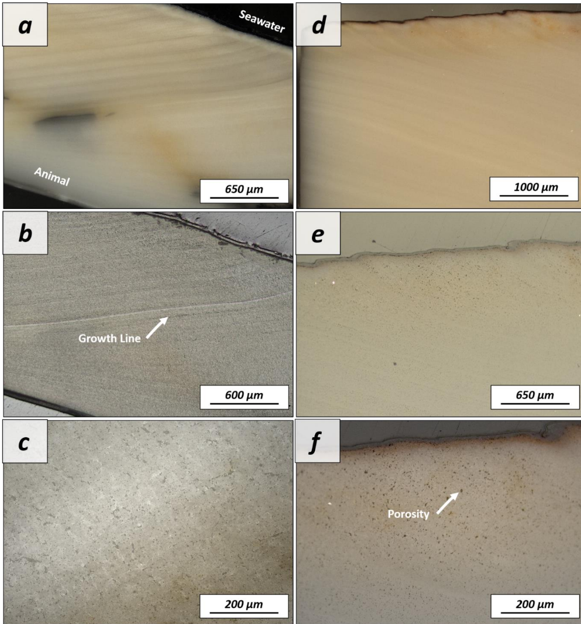
1135 Figure A4. Laser confocal microscopy images of (a-c) pristine and (d-f) altered shells of Arctica islandica . The shells display a homogeneous internal structure where porosity and growth lines can be observed. After 6 months of hydrothermal alteration, major changes to the shell structure cannot be observed with laser confocal microscopy imaging.
