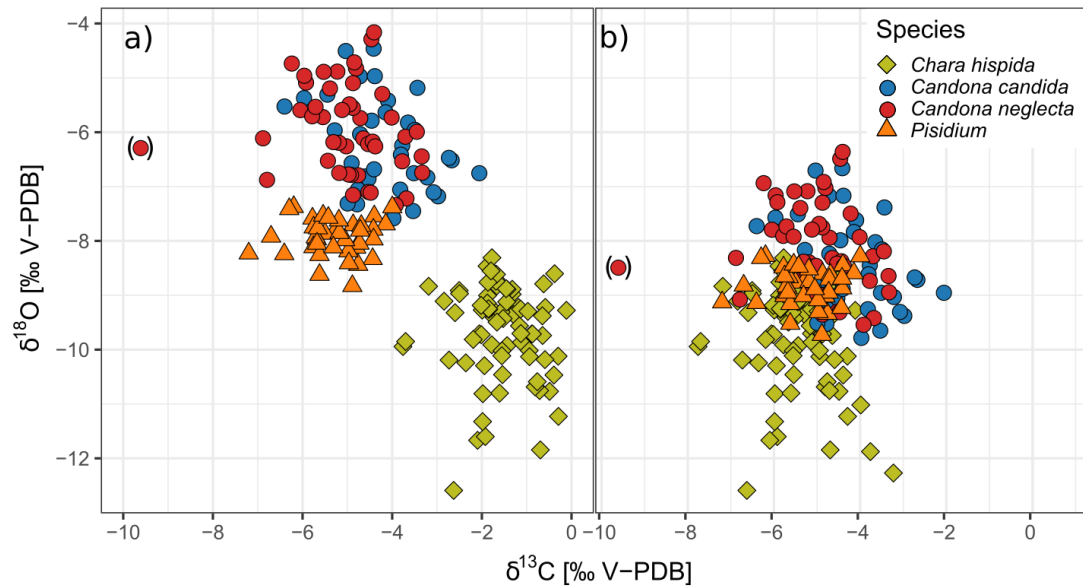
Figure 6. Isotopic composition of specific biogenic carbonate samples collected from surface sediments and living organisms and from subfossil remains in surface sediments of Lake Locknesjön. a) \delta^{18}\text{O} and \delta^{13}\text{C} of calcite encrustations from Chara hispida and of valves from Candona candida , Candona neglecta and Pisidium . b) The same data with published vital offsets corrected for: \delta^{13}\text{C} Chara hispida : -4‰ (value from Hammarlund and Keen, 1994), \delta^{18}\text{O} ostracods: -2.2‰, \delta^{18}\text{O} Pisidium : -0.9‰ (values from von Grafenstein et al., 1999b). The data point marked in brackets was identified as a major outlier and left out from further analysis and figures.
