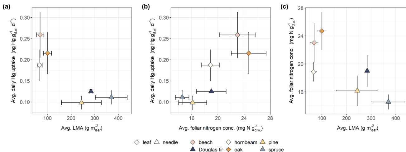
Figure 4. a) Average daily Hg uptake rates (ng Hg g -1 d.w. d -1 ), b) average foliar nitrogen concentrations (mg N g -1 d.w.) and c) average LMA (g d.w. m -2 leaf) determined in 338-349 foliage samples and resolved by tree species group and foliage type (leaf/needle). Error bars denote \pm one standard deviation. Number of samples (n) differs between tree species: beech (n = 164), Douglas fir (n = 2), hornbeam (n = 9), oak (n = 106), pine (n = 2435) and spruce (n = 33).
