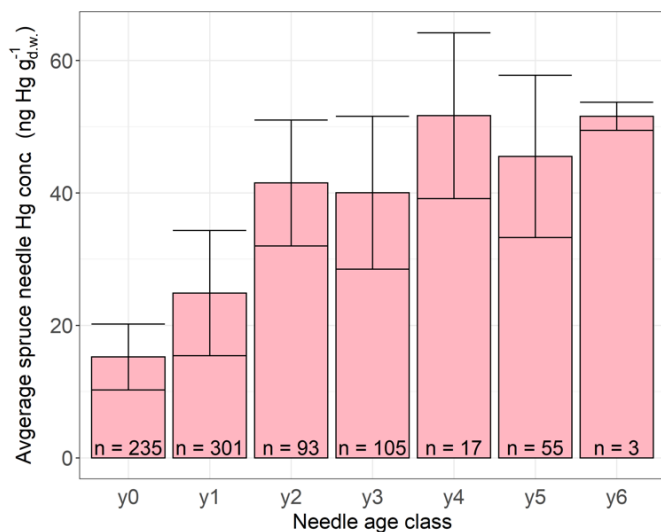
Figure 7. Average Hg concentrations (ng Hg g d.w. -1 ) in spruce needle samples of different ages. Needle age class y 0 corresponds to current-season needles developed flushed in the year of sampling, y 1 corresponds to one-year old needles, y 2 corresponds to two-year old needles etc. Error bars denote ± one standard deviation between multiple samples, n indicates number of samples.
