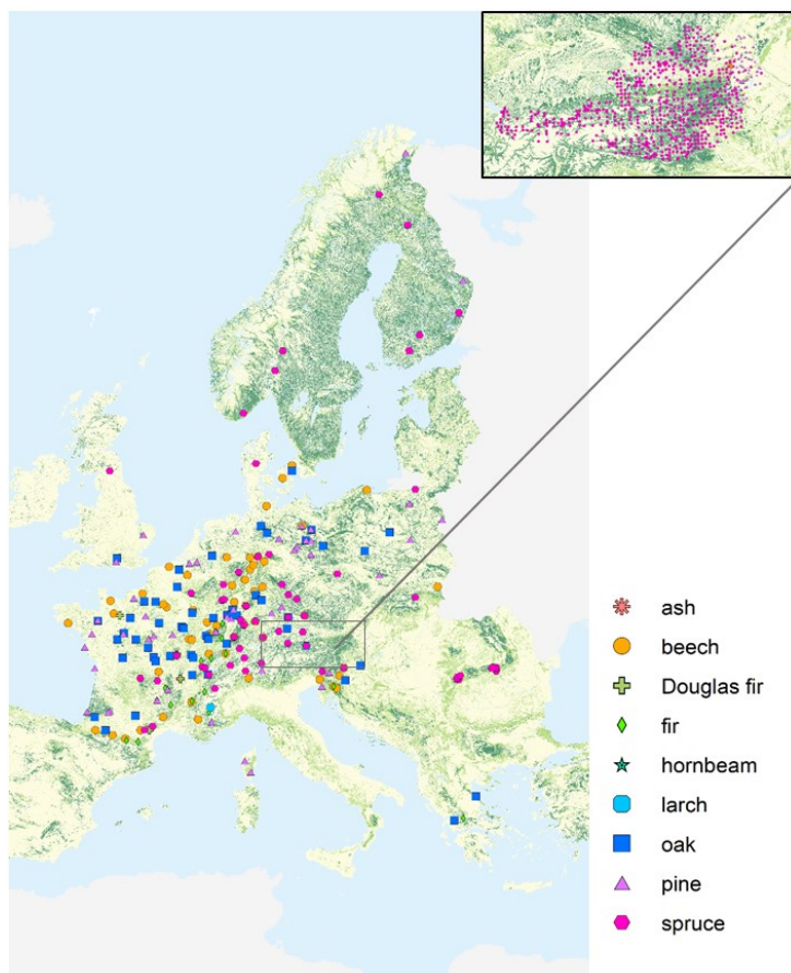
140 Figure 1. Overview of forest plots, at which Hg foliage samples were harvested from different tree species groups during the sampling year 2017. At around 12% of plots in 2017, foliage from more than one tree species group was sampled. Geographic distribution of sampling sites in 2015 is similar, except there were no samples from the ICP Forests countries-partners Brandenburg (Germany), Baden-Württemberg (Germany) and Poland and there were samples from five additional plots in North Rhine-Westphalia (Germany), see Fig. S1. The enlarged map view at the top right depicts sampling locations of the Bio-Indicator Grid in Austria in 2015 and 2017. Use of base map authorized under European Commission reuse policy (EU, 2011).
