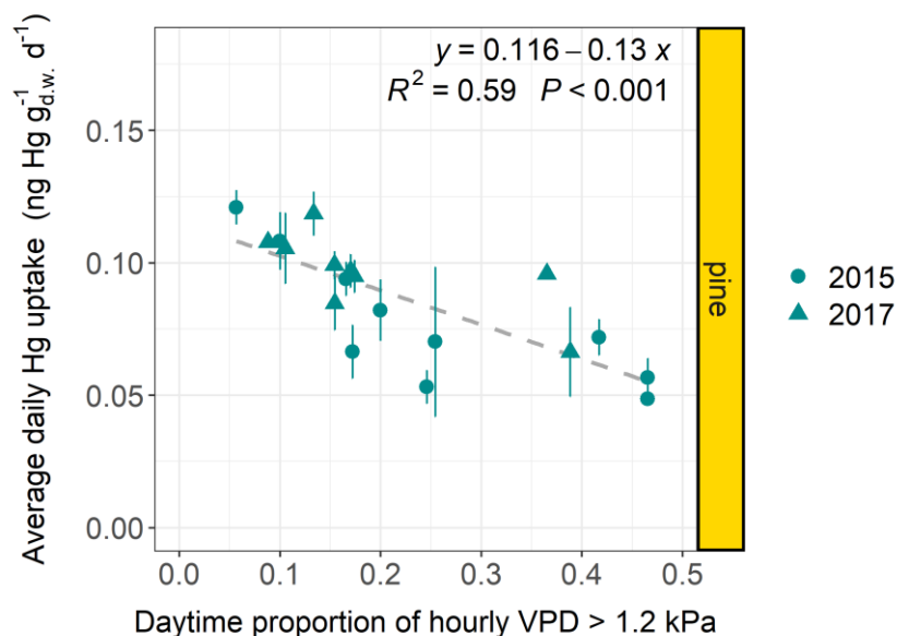
Figure 5. Average daily Hg uptake rates (ng Hg g -1 d.w. d -1 ) of (a) current-season pine and (b) current-season spruce needles from multiple forest plots (pine plots n = 19; spruce plots n = 14) versus the proportion of daytime hours (06:00 – 18:00 LT) within an average day of the respective sample life periods, during which the hourly daytime water vapor pressure deficit (VPD) exceeded a threshold value of (a) 1.2 kPa and (b) 3 kPa. Data points originate from both sampling years 2015 and 2017. All forest plots are located in Central Europe (latitude 46° - 54°), for which ambient air Hg(0) concentrations are relatively constant (see Table S2 and Fig. S6). Error bars denote ± one standard deviation of daily needle Hg uptake rates between multiple samples at each forest plot.
