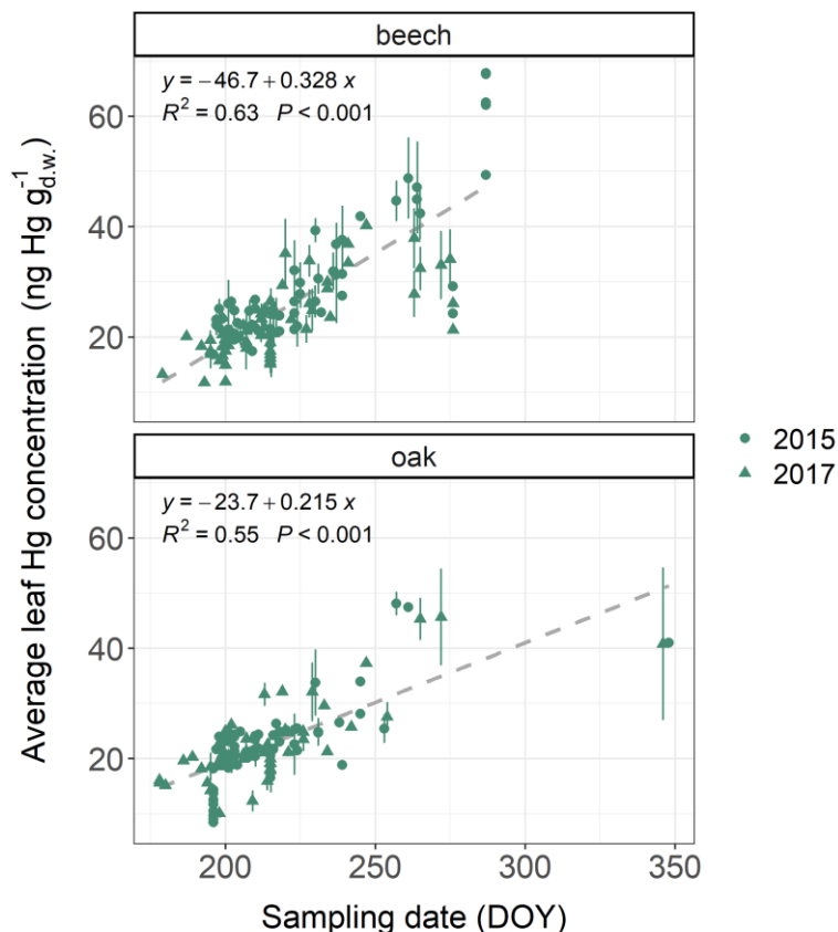
265 Figure 2. Average leaf Hg concentrations ( \text{ng Hg g}^{-1}_{\text{d.w.}} ) in beech and oak samples at multiple ICP Forests plots versus sampling dates (day of year; DOY) of respective samples. Sampling took place both in 2015 and 2017. Two plots of holm oak ( Quercus ilex ) are located in Greece and were sampled in December 2015 (DOY = 348) and December 2017 (DOY = 346). Error bars denote \pm one standard deviation between multiple samples at each forest plot.
