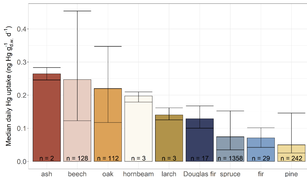
315 Figure 3. Median daily foliar Hg uptake (ng Hg g -1 d.w. day -1 ) between different tree species groups (see Table S1 for definition of tree species groups) arranged from highest to lowest value. Error bars give the value range within each tree species group and n indicates the number of sites at which the respective tree species were sampled in both the years 2015 and 2017. Foliar samples of evergreen coniferous tree species (Douglas fir, spruce, fir and pine) consist of needles of the current season.
