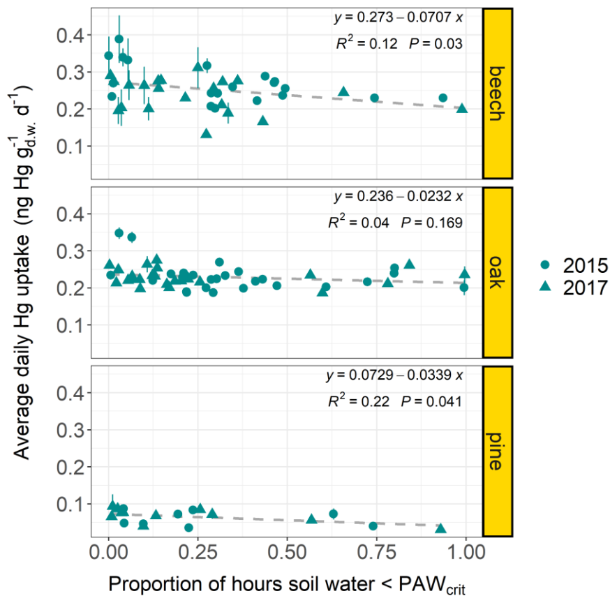
Figure 6. Average daily Hg uptake rates (ng Hg g -1 d.w. d -1 ) of beech, oak and current-season pine foliage from multiple forest plots (beech plots n = 38; oak plots n = 45; pine plots n = 19; latitude: 41° - 55° ) versus the proportion of hours within the respective sample life periods, during which the geographically associated hourly soil water from the ERA5-Land dataset (Muñoz Sabater, 2019) fell below a soil texture specific threshold value PAW crit (see Sect. 2.6). Data points originate from both sampling years 2015 and 2017. Error bars denote ± one standard deviation of daily needle Hg uptake rates between multiple samples at each forest plot.
