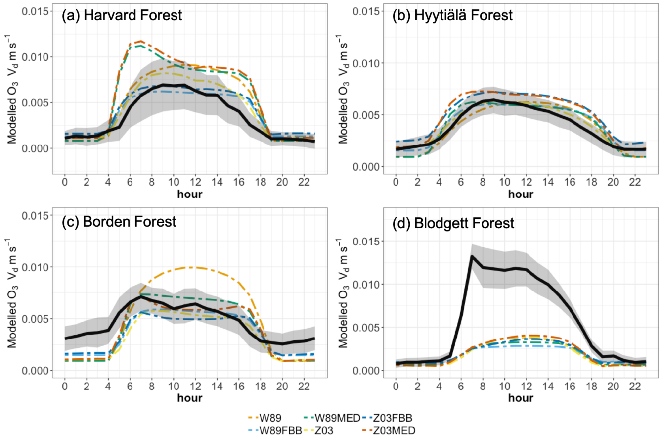
405 Figure 3. Average diurnal cycles of ozone dry deposition velocity at four long-term observational sites. Black solid lines indicate observed average diurnal cycles of v_d . Shaded envelope indicates standard deviation of summertime average hourly v_d . Dashed lines indicate simulated diurnal cycles of v_d using different dry deposition schemes.
