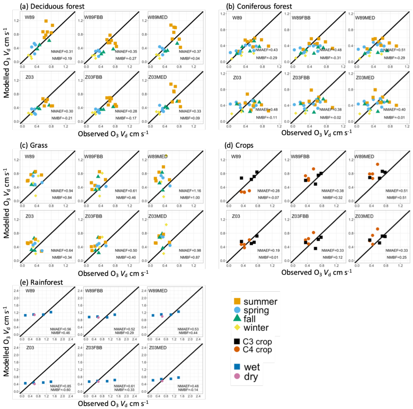
330 Figure 1. Average daytime (LT 6:00~18:00) observed and simulated dry deposition velocities for five land types. Each data point refers to seasonal average daytime O_3 dry deposition velocity from one dataset listed in Table S1. Colors indicate dominant seasons during field measurements, except that for crops where different colors indicate crop types (C3 and C4 crops).
