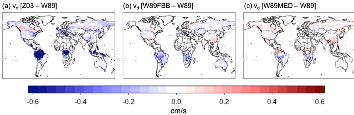
580 Figure 10. Differences in average daytime v_d between different dry deposition schemes for 2010-2014 July.
