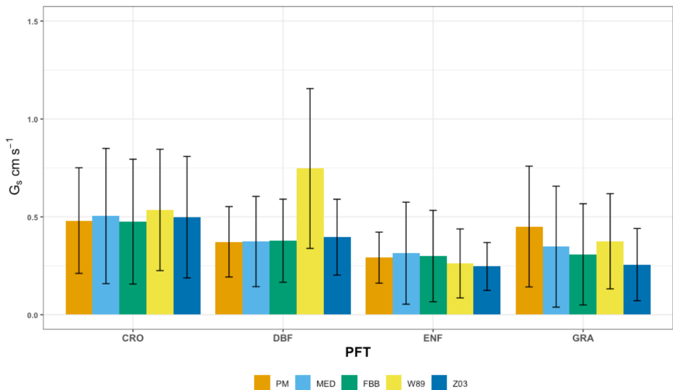
Figure 8. Average daytime canopy stomatal conductance ( G_s ) computed with different stomatal conductance approaches for the four major PFTs. The error bars indicate two standard deviations. DBF: Deciduous Broadleaf Forest; ENF: Evergreen Needleleaf Forest; CRO: Crop; GRA: Grass.
