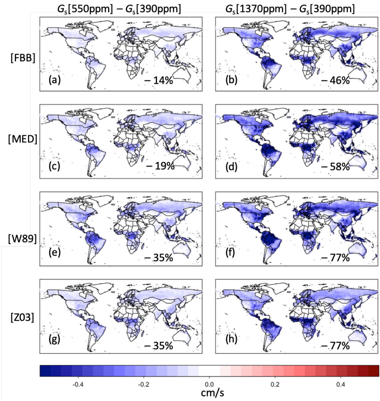
Figure 12. Changes in July daytime average G_s , simulated with FBB, MED and W89 (using empirical CO 2 response function) under different CO 2 levels.
