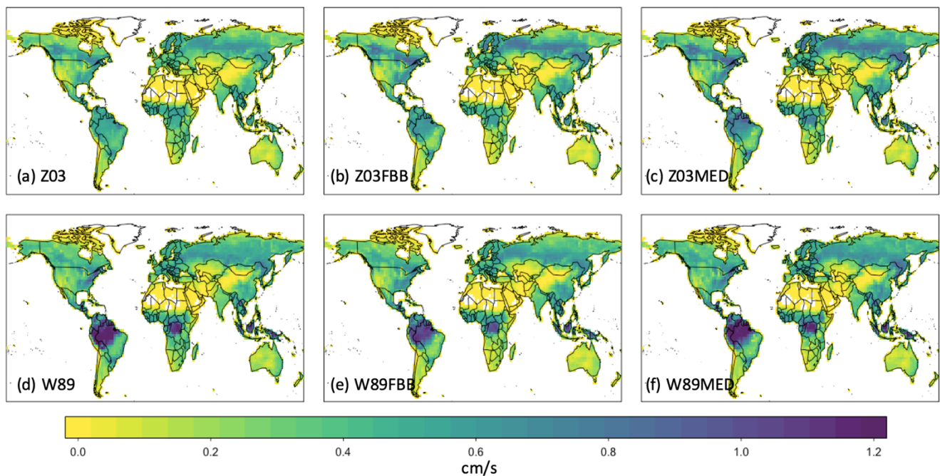
Figure 9. 2010–2014 July average daytime v_d under 390 ppm CO 2 level simulated with the six dry deposition schemes: (a) Z03, (b) Z03FBB, (c) Z03MED, (d) W89, (e) W89FBB, (f) W89MED.
