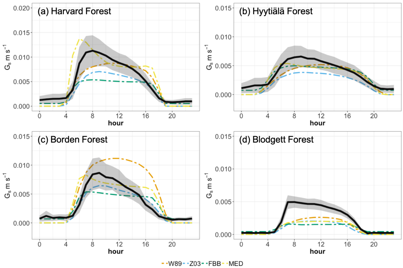
410 Figure 4. Simulated and observed diurnal cycles of canopy stomatal conductance for ozone during summer at the four long-term measurement sites. Black lines indicate G_s derived with P-M method. Shaded envelope shows standard deviation of summertime average hourly G_s . Colored solid lines indicate simulated stomatal conductance using multiplicative and photosynthesis-based stomatal approaches.
