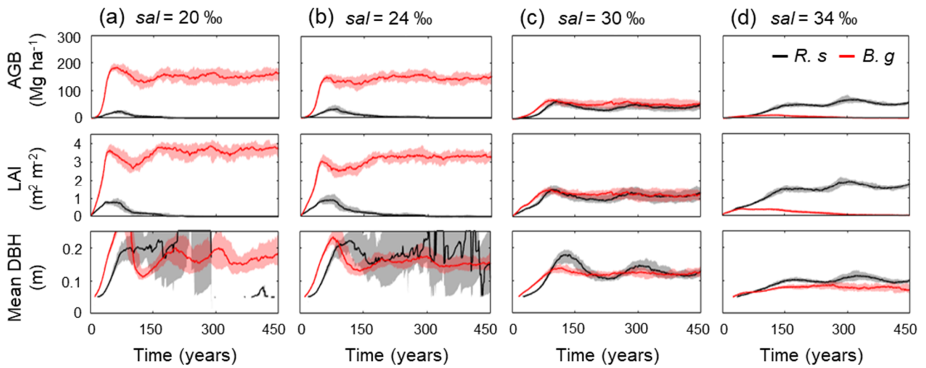
Figure 76. Temporal dynamics in above-ground biomass (AGB), leaf area index (LAI), and mean diameter at breast height (DBH) of R. stylosa ( R. s ) and B. gymnorhiza ( B. g ) in four soil salinity conditions (a) 20‰, (b) 24‰, (c) 30‰, and (d) 34‰. Note that trees with DBH < 0.05 m were not included in the calculation of mean DBH. Solid lines show median and shading the 90-th percentile from ensemble simulations.
