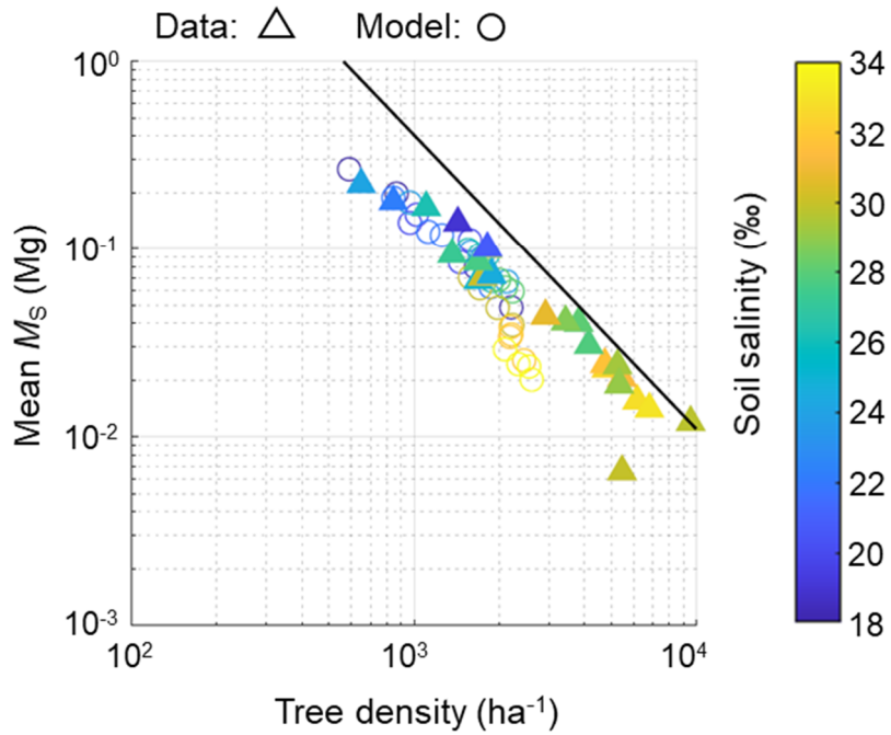
455 Figure 98. The relationship of tree density and mean individual stem biomass ( M_s ). Triangles show field data while circles show modeled values from one of the ensemble simulations with different soil salinity settings (from 18‰ to 34‰ with 2‰ increments) plotted from 300–450 years (with interval of 50 years), which is in steady states in terms of forest structural
