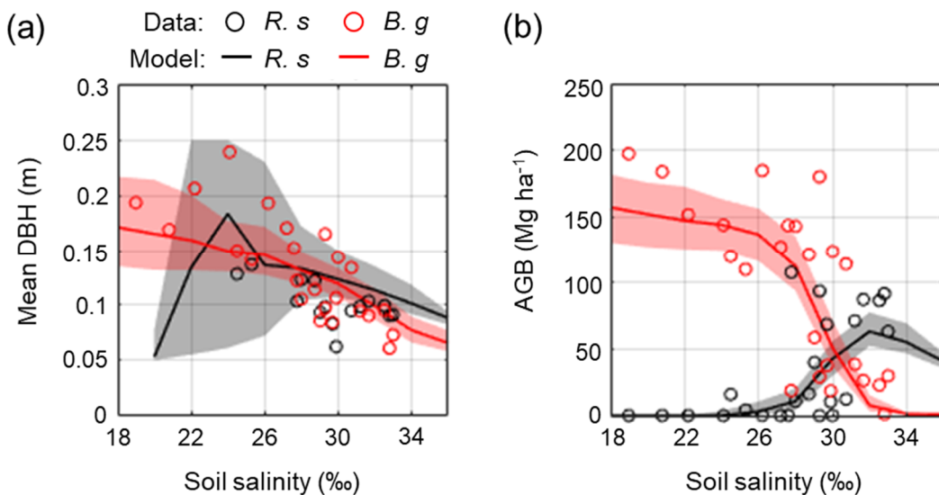
Figure 87. Comparison of field-measured and modeled (a) mean DBH and (b) AGB of R. stylosa and B. gymnorhiza along with soil salinity gradient. From each ensemble simulation, modeled mean DBH and AGB in steady states (> 300 years)
