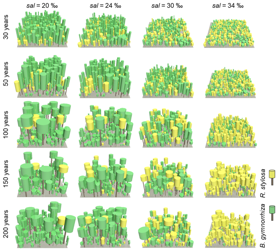
405 Figure 6.5. Visualization of forest structures over 200 years under different soil salinity ( sal ), 20, 24, 30, and 34‰, taken from one of the ensemble simulations. The brown-colored objects represent the stem the while the yellow orange and or green-colored objects represent the crowns of R. stylosa and B. gymnorhiza , respectively. The forest floor shown is the 30 m × 30 m-wide computational domain.
