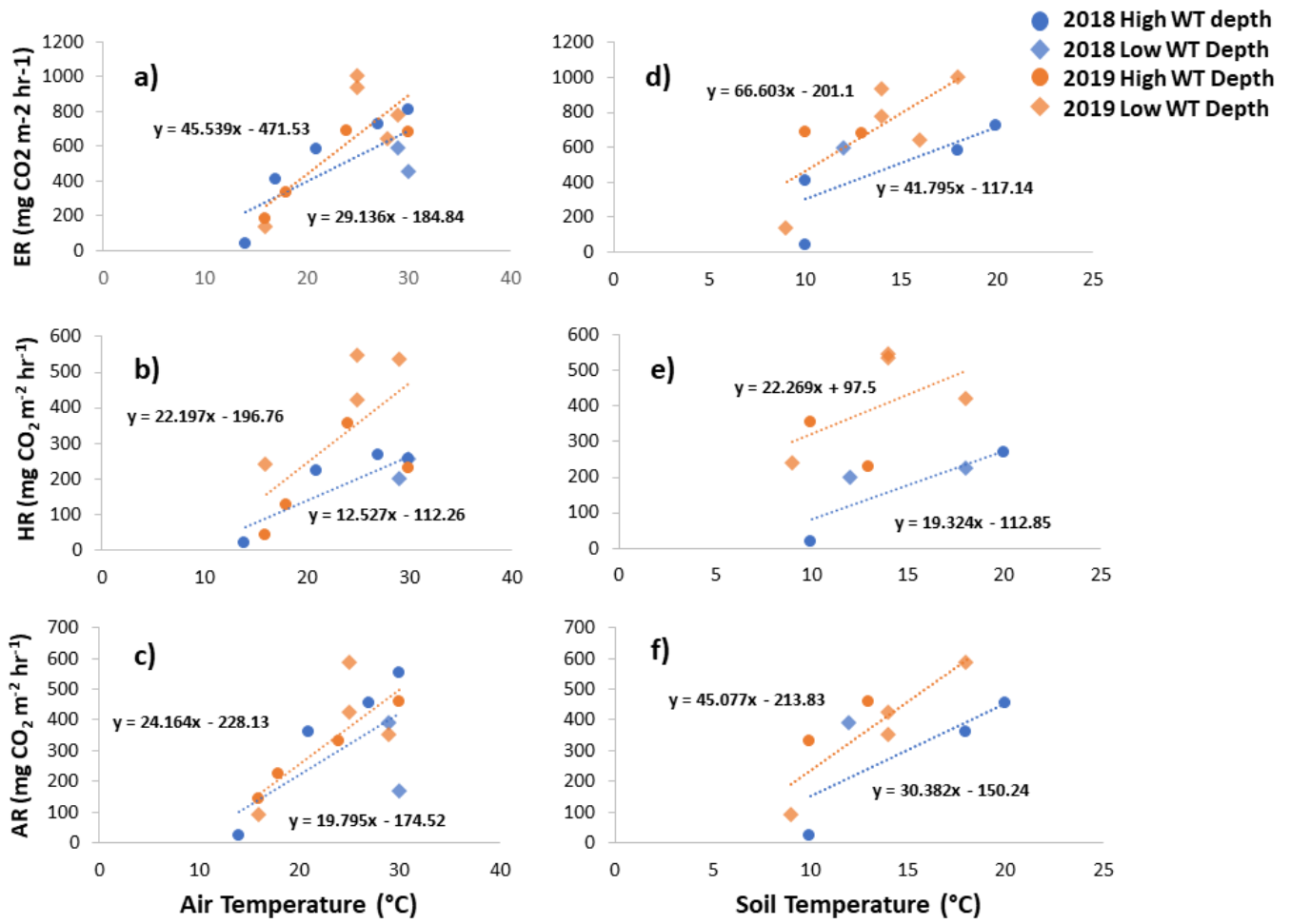
Figure 7. Scatterplots with trend lines of relationships between air temperature and a) ER, b) HR, and c) AR; and between soil temperature and d) ER, e) HR, and f) AR in the sedges across the growing seasons of 2018 and 2019. High WT refers to water table positions from surface to 35 cm depth.
