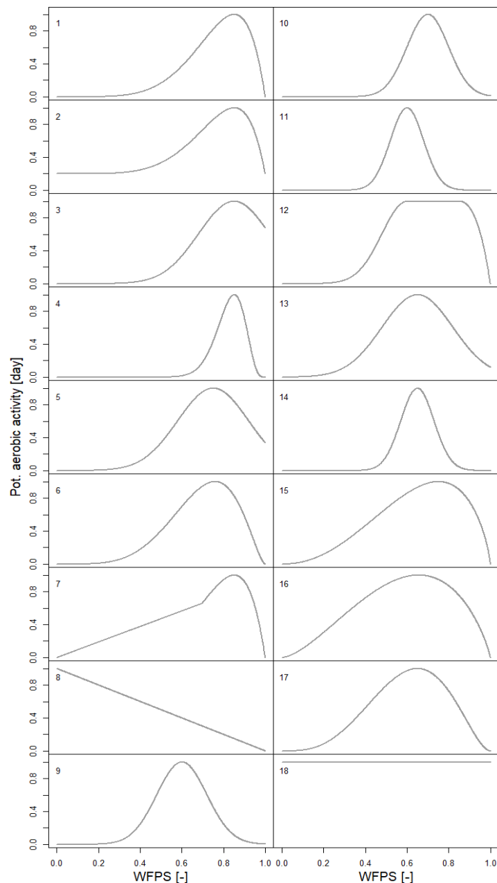
340 Figure 4 –The ensemble of WFPS optimum curves that was tested during model optimization.
