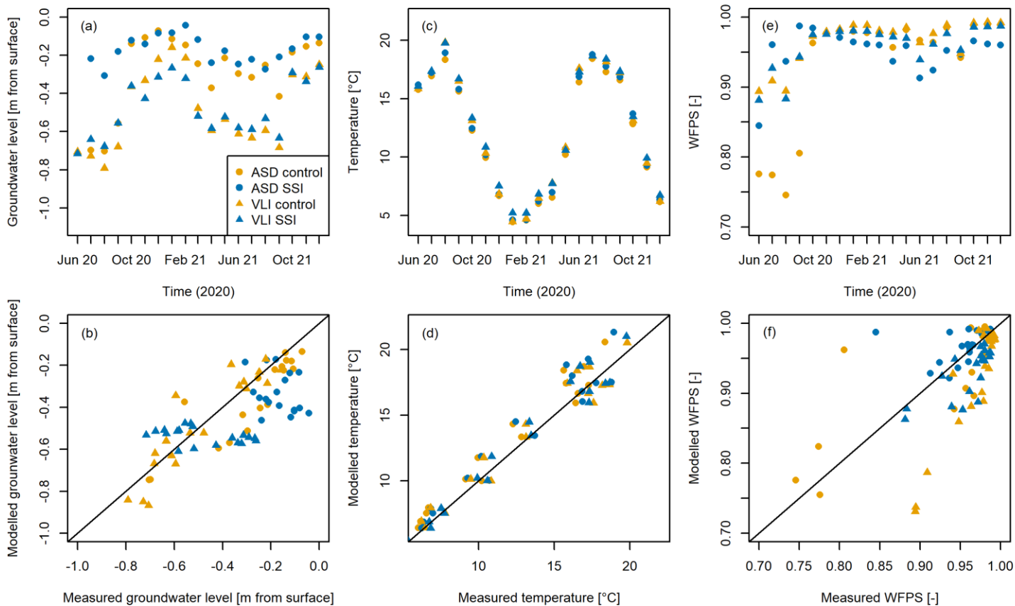
385 Figure 5 – Monthly averages of measured (a) groundwater level, (c) soil temperature and (e) WFPS that are compared with monthly modelled averages of (b) groundwater level, (d) temperature and (f) WFPS. Values for temperature and WFPS were averaged over a depth of 0.4 m. The legend in (a) applies for all panels.
