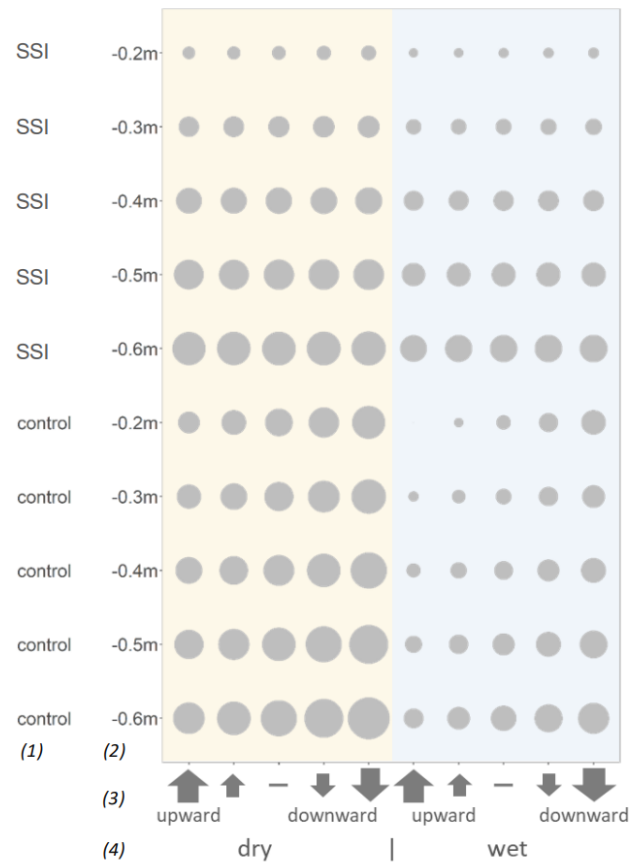
Figure 8 – (a) Dot graph of calculated potential respiration rate over the complete width of the model domain. Model runs are distinguished by (1) application of SSI, (2) ditch water level from surface, (3) hydrological regime (1 mm d-1 upward to downward flow across the bottom boundary) and (4) meteorology (2018 for dry, 2012 for wet). (b) Effects of SSI (above) and ditch water level (below) on respiration rate. Green dots represent a decrease in respiration rate. Effects of SSI were determined by comparing similar model runs with and without SSI. Effects of ditch water level were determined by comparing each scenario in which the water level is 0.5 m below surface with the other scenarios in the same category on the x-axis.
