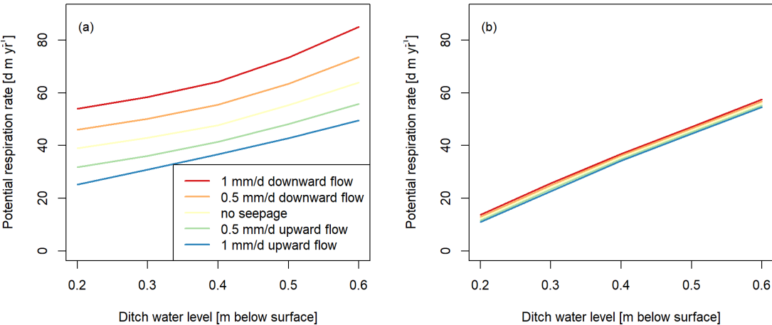
535 Figure 9 – (a) The simulated effects of ditch water level on potential respiration rate for different seepage settings within a control scenario and (b) these effects with SSI in the dry year 2018. The colors of the lines represent the model seepage setting.
