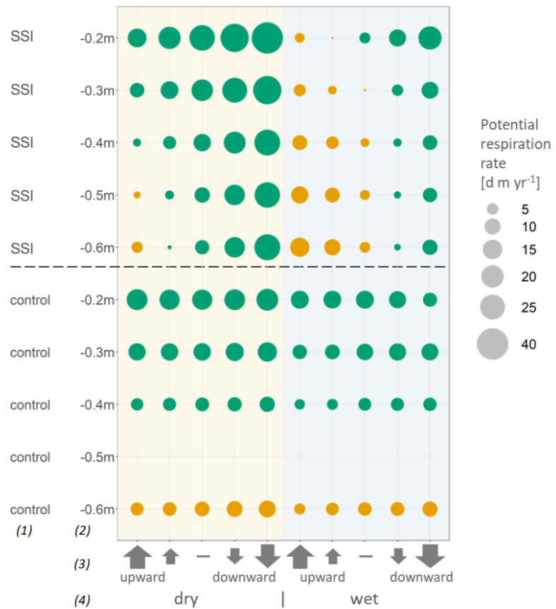
Figure 8 – (a) Dot graph of calculated potential respiration rate over the complete width of the model domain. Model runs are distinguished by (1) application of SSI, (2) ditch water level from surface, (3) hydrological regime (1 mm d-1 upward to downward flow across the bottom boundary) and (4) meteorology (2018 for dry, 2012 for wet). (b) Effects of SSI (above) and ditch water level (below) on respiration rate. Green dots represent a decrease in respiration rate. Effects of SSI were determined by comparing similar model runs with and without SSI. Effects of ditch water level were determined by comparing each scenario in which the water level is 0.5 m below surface with the other scenarios in the same category on the x-axis.
