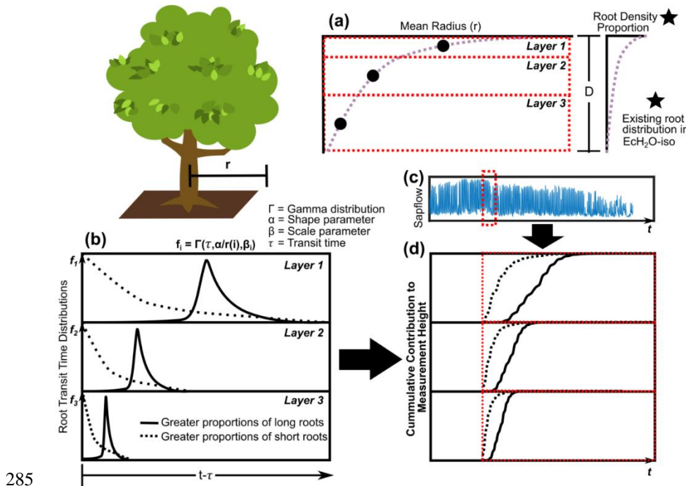
Figure 2: The estimation of rooting density (a) vertically and (b) the transit time distribution describing root velocity and distance to measurement height weighted by (c) sap flow to get the (d) cumulative contribution of soil water from entry time (red line).
