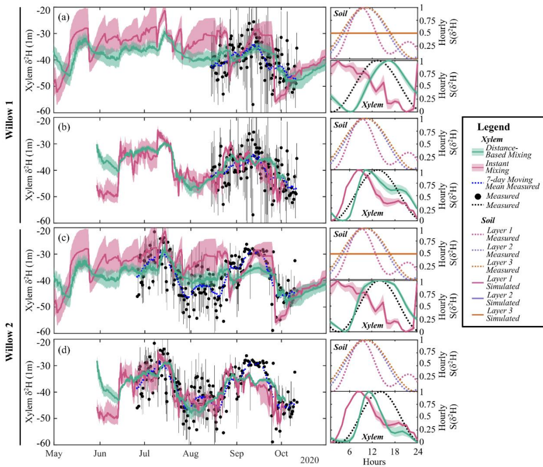
470 Figure 6: Simulated 12-hour average xylem deuterium using (a) simulated and (b) measured soil deuterium with distance-based and instant mixing in Willow 1. Simulated 12-hour average xylem deuterium using (c) simulated and (d) measured soil deuterium with distance-based and instant mixing in Willow 2. Measurement bars represent the maximum and minimum measured xylem water isotopes during the 12-hour period. For each simulation, standardized sub-daily \delta^2\text{H} ( S(\delta^2\text{H}) ) shows the measured and simulated soil (cell contribution weighted average) and xylem average hourly variability. Note: standardized simulated soil water isotopes overlap for all soil layers.
