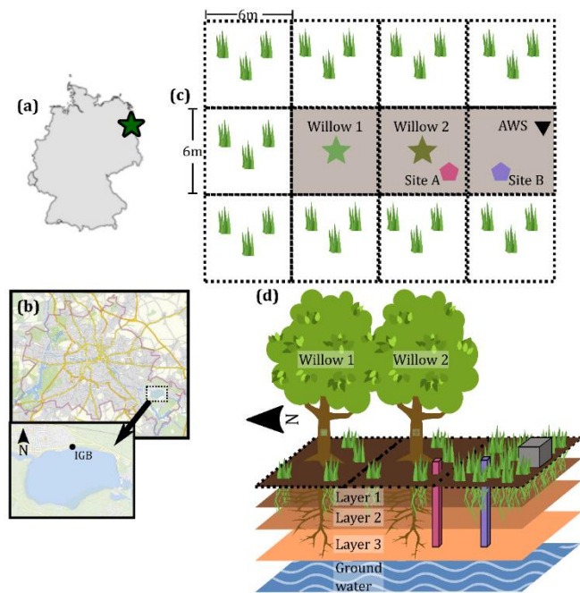
100 Figure 1: Study site location and site description. (a) Location of the site within Germany, (b) Location of IGB within Berlin (Berlin, 2021), (c) plan view of the study site including the location of willow trees, soil water isotope and moisture, and automatic weather station (AWS), and (d) conceptual diagram of the study site, with three soil depths and two primary vegetation units (with relative 105 prominence). Pink and blue columns in subplot d indicate soil moisture and isotope measurement columns, and grey box indicates AWS location. Berlin Maps © OpenStreetMap contributors 2021. Distributed under the Open Data Commons Open Database License (ODbL) v1.0. The area surrounding the study site is grass-covered, similar to Site B.
