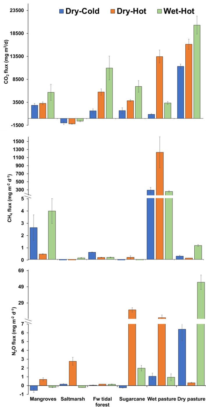
Figure 2: Greenhouse gas fluxes of ( \text{mg m}^{-2} \text{d}^{-1} ) (a) CO 2 (b) CH 4 and (c) N 2 O from the soils of tropical coastal wetlands: mangroves, saltmarsh, freshwater (Fw) tidal forest, and two alternative land uses: sugarcane and pastures (wet and dry) during three periods of the year: dry-cold, dry-hot and wet-hot
